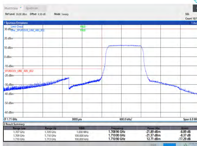
Band66-1.4MHz-QPSK-131979-6RB#0
