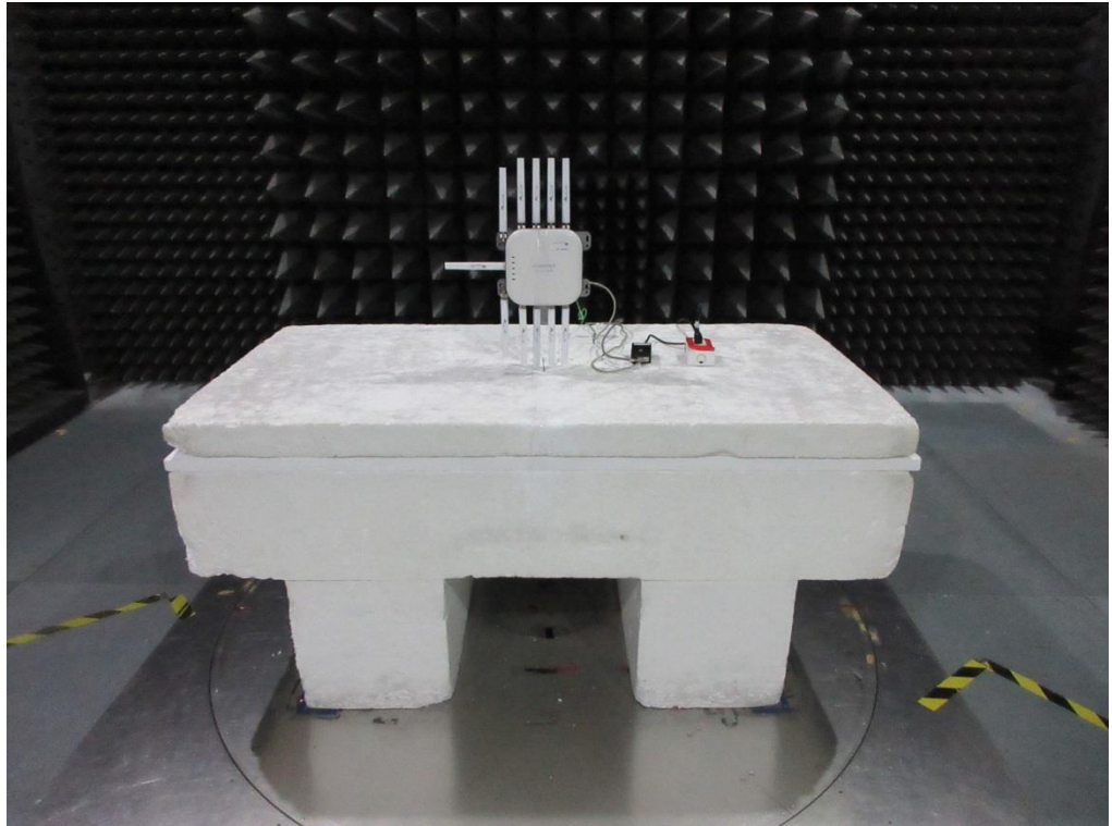
Beamforming Radio 1
