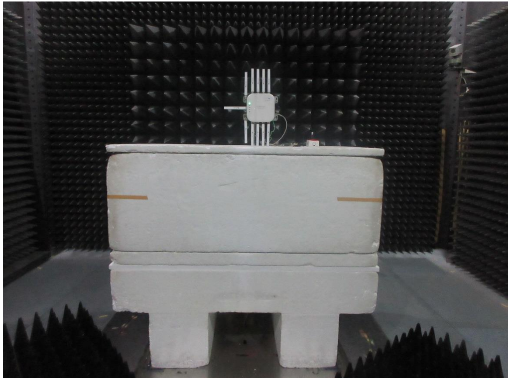
Beamforming Radio 3
