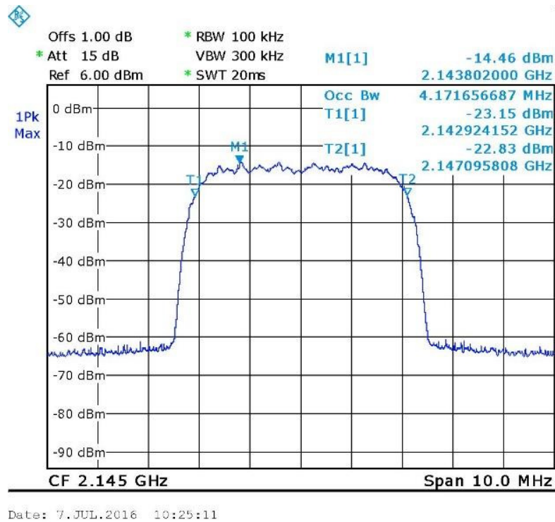
Figure 36. — W-CDMA (2145.0MHz) IN
