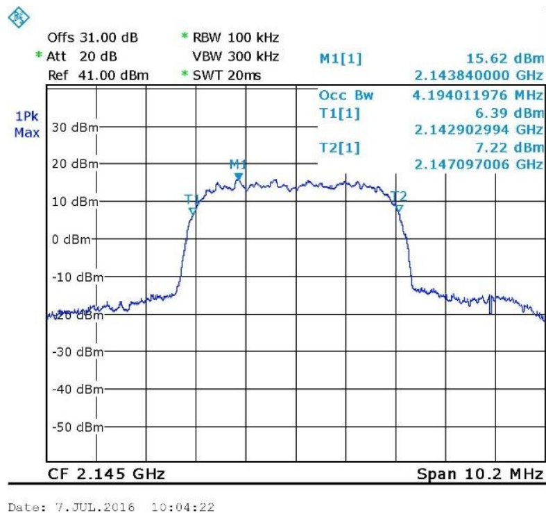
Figure 37. — W-CDMA (2145.0MHz) OUT
