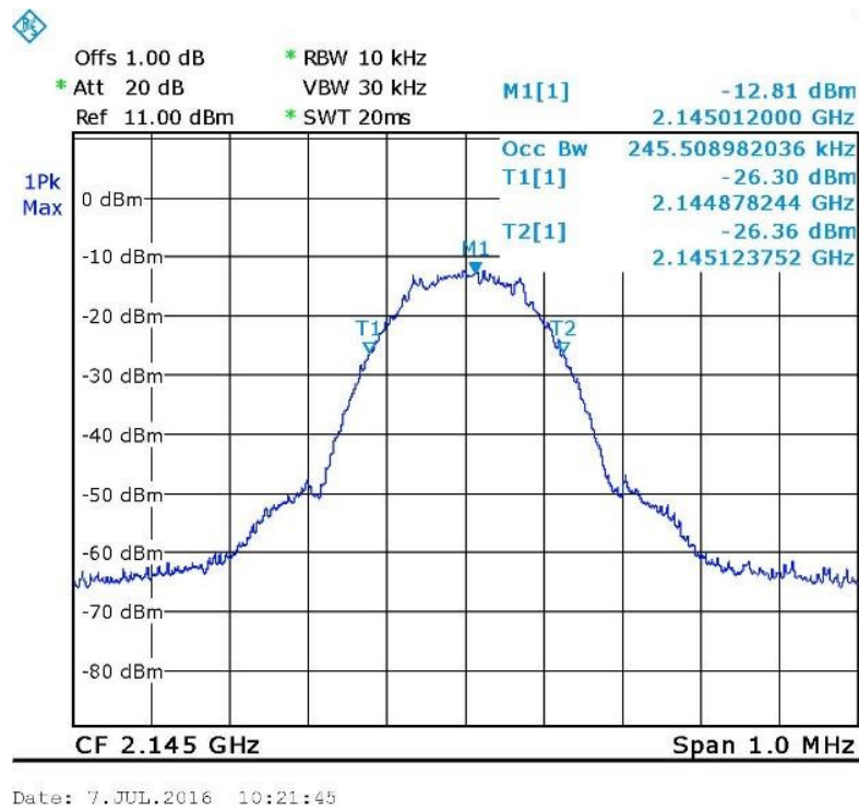
Figure 30. — GSM (2145.0MHz) IN
