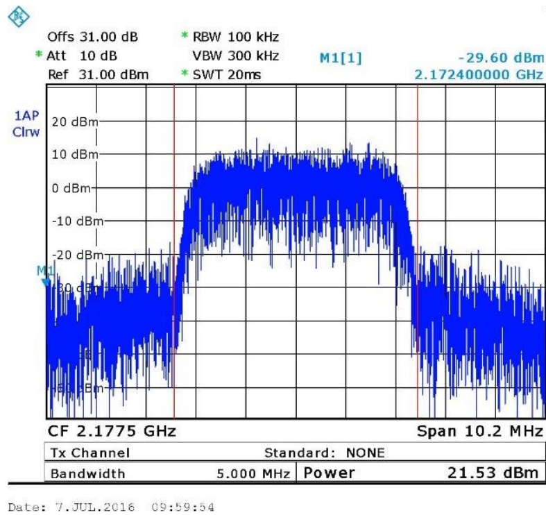
Figure 19. — W-CDMA (2177.5MHz)
