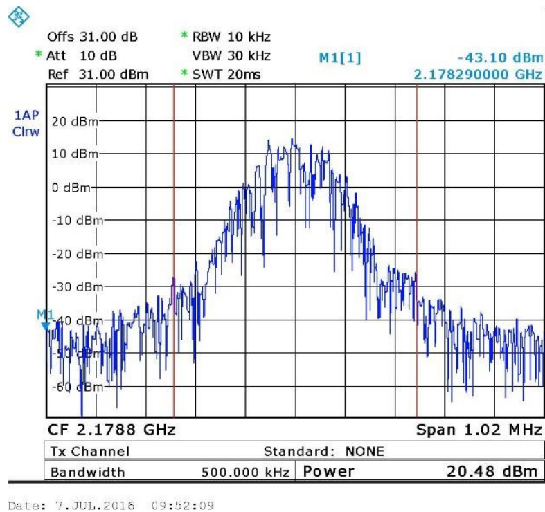
Figure 13. — GSM (2178.8 MHz)
