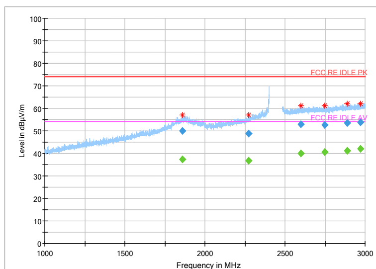
Fig 60. Radiated Spurious Emission (802.11b,Ch1,1GHz~3GHz)
