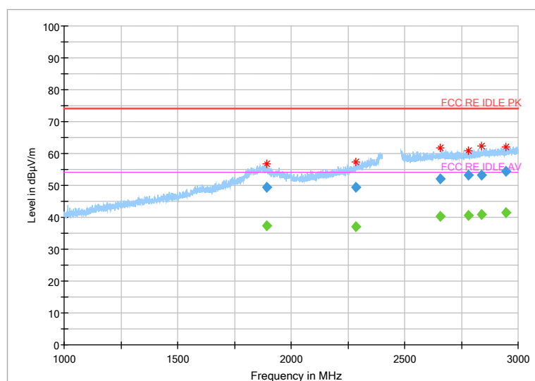
Fig 70. Radiated Spurious Emission (802.11 n-20MHz,Ch1,1GHz~3GHz)
