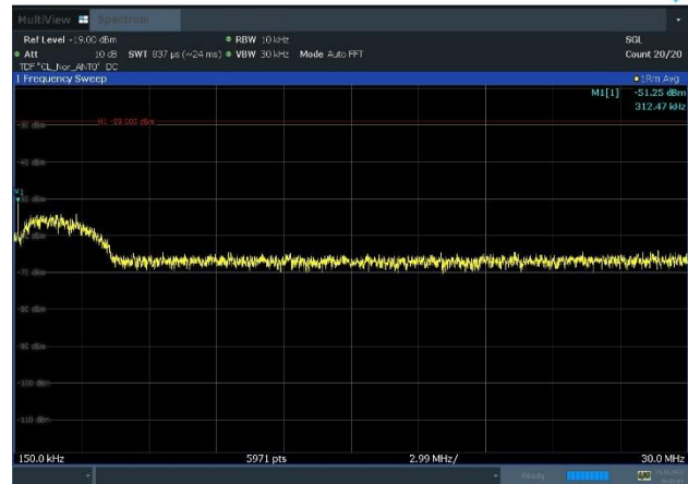
Plot 8-18. Conducted Spurious Emission Plot 150 kHz to 30 MHz (n26_1C_5M+n29_1C_5M+n71_1C_5M_QPSK – Mid, Port 0)
