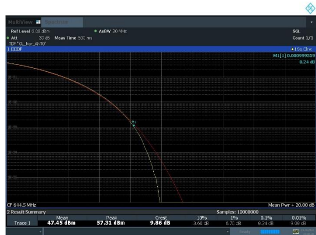
Plot 8-8. Peak To Average Power Ratio Plot (n71_1C_15M_16QAM - High Channel, Port 0)
