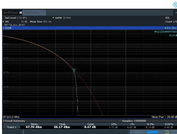
Plot 8-7. Peak To Average Power Ratio Plot (n71_1C_15M_QPSK - Low Channel, Port 0)
