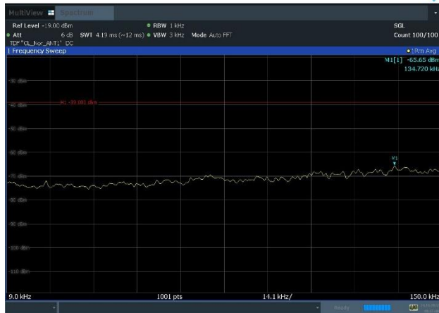
Plot 8-11. Conducted Spurious Emission Plot 9 kHz to 150 kHz (n71_1C_15M_QPSK - Low Channel, Port 1)
