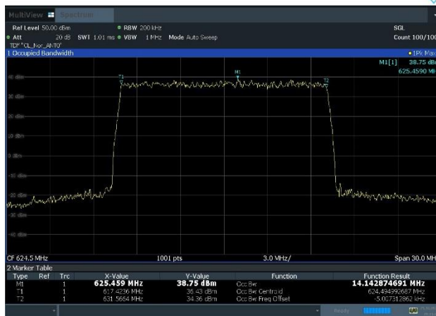
Plot 8-1. Occupied Bandwidth Plot (n71_1C_15M_QPSK - Low Channel, Port 0)
