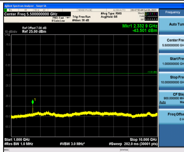
Band13-10MHz-QPSK-23230-1-0-Low-1000-10000--43.5-PASS
