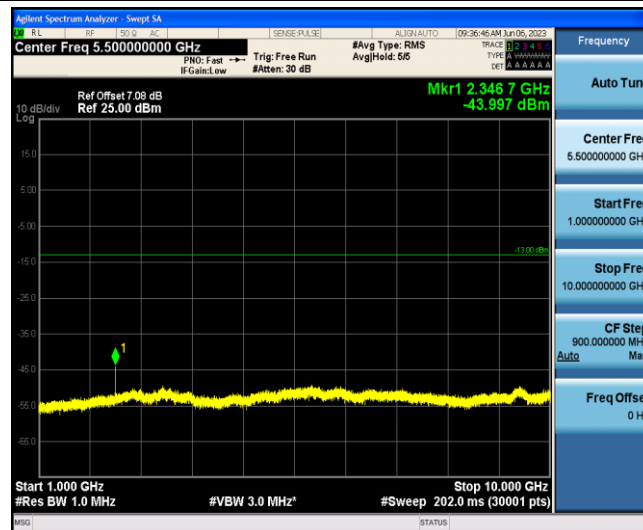
Band13-5MHz-16QAM-23255-1-0-Low-1000-10000--44-PASS
