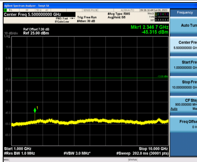
Band13-5MHz-QPSK-23255-1-0-Low-1000-10000--45.32-PASS
