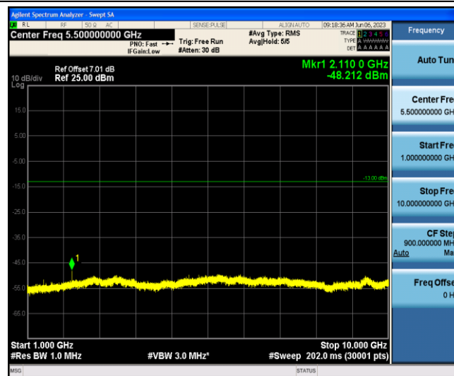
Band12-10MHz-QPSK-23095-1-0-Low-1000-10000--48.21-PASS
