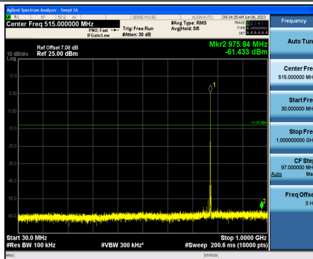
Band13-5MHz-16QAM-23205-1-0-Low-30-1000--61.43-PASS
