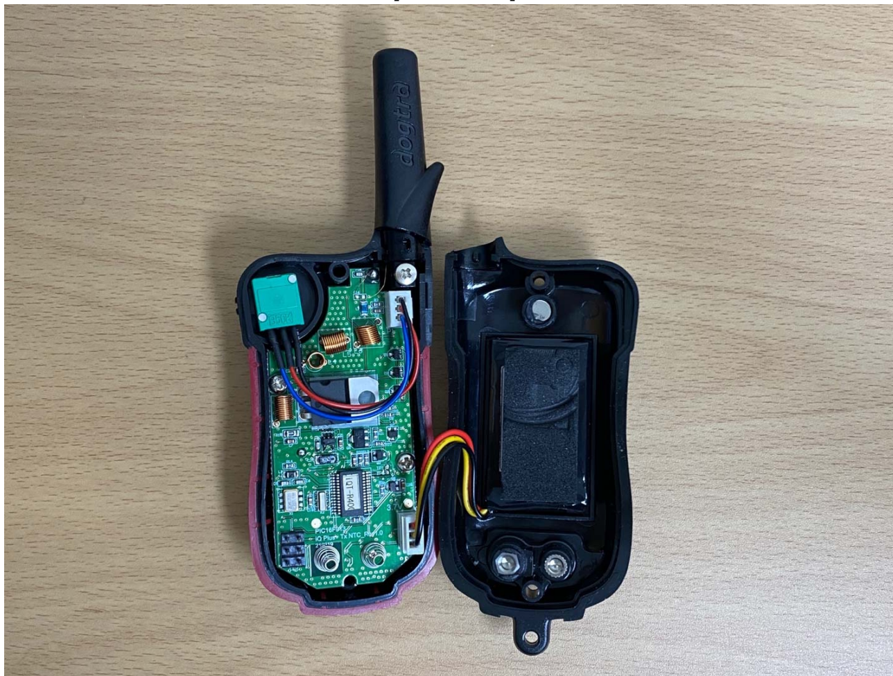
[ Inside View ]
