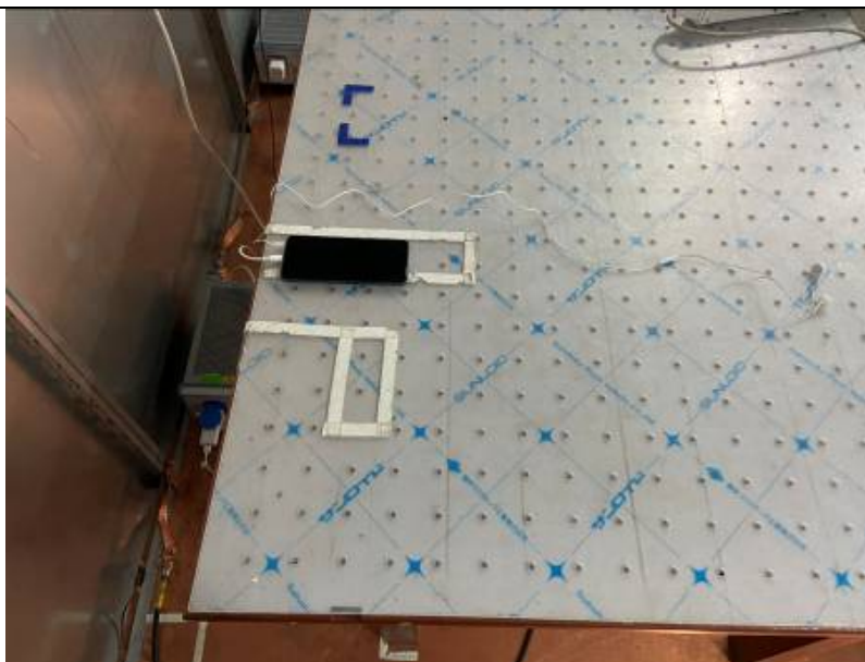
Conducted Emissions Test Setup (with charger)
