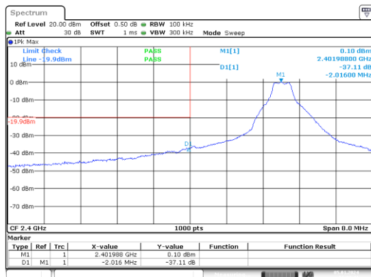
GFSK_Low
