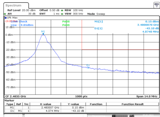
GFSK_High
