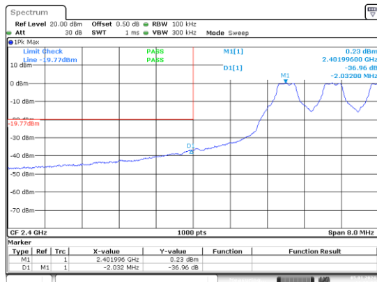
GFSK_Hopping_Lower
