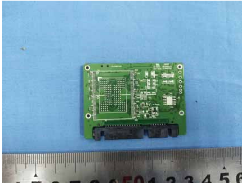
EUT –SSD Board Bottom View
