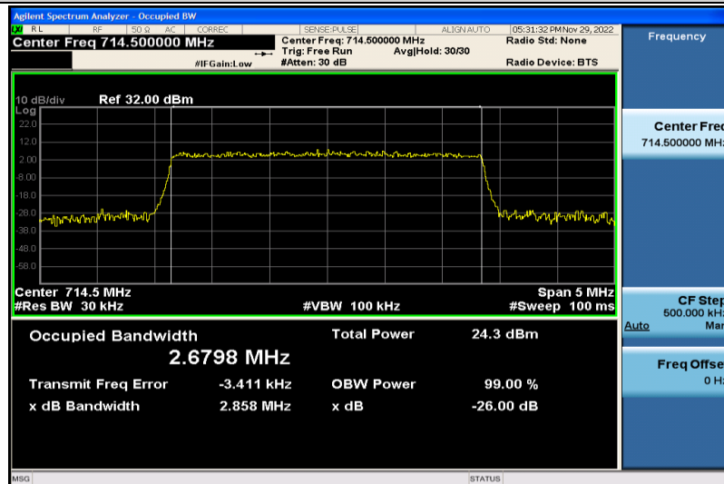
Band12-3MHz-64QAM-23165-15RB#0-2.6798
