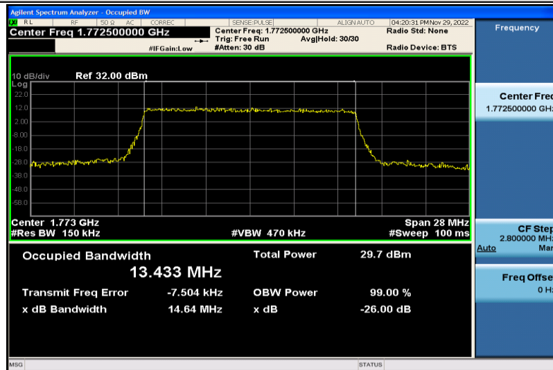
Band66-15MHz-QPSK-132597-75RB#0-13.433
