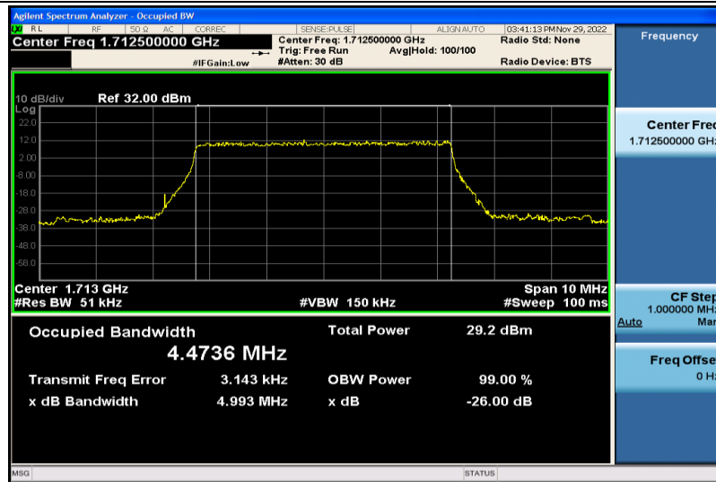
Band66-5MHz-QPSK-131997-25RB#0-4.4736
