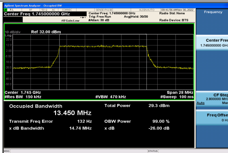
Band66-15MHz-64QAM-132322-75RB#0-13.450
