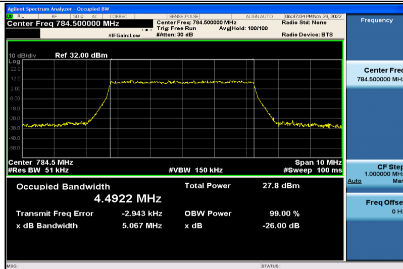
Band13-5MHz-64QAM-23255-25RB#0-4.4922
