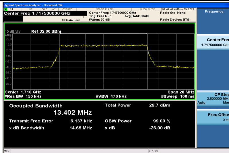
Band66-15MHz-64QAM-132047-75RB#0-13.402
