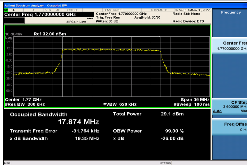
Band66-20MHz-64QAM-132572-100RB#0-17.874
