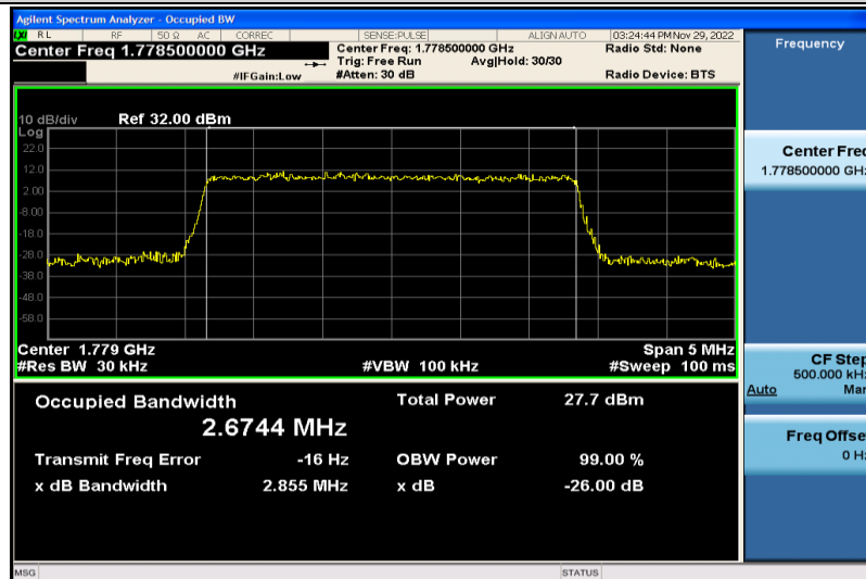
Band66-3MHz-16QAM-132657-15RB#0-2.6744
