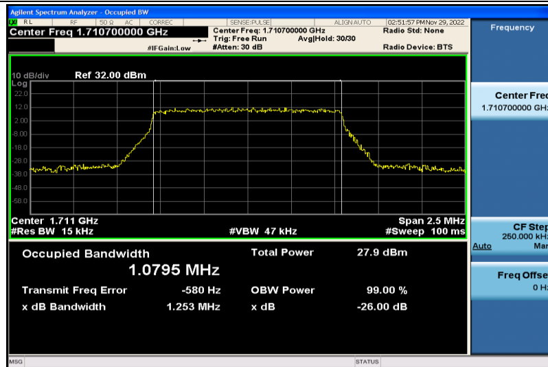
Band66-1.4MHz-QPSK-131979-6RB#0-1.0795
