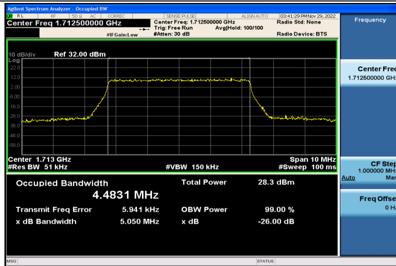
Band66-5MHz-16QAM-131997-25RB#0-4.4831
