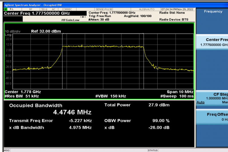
Band66-5MHz-64QAM-132647-25RB#0-4.4746
