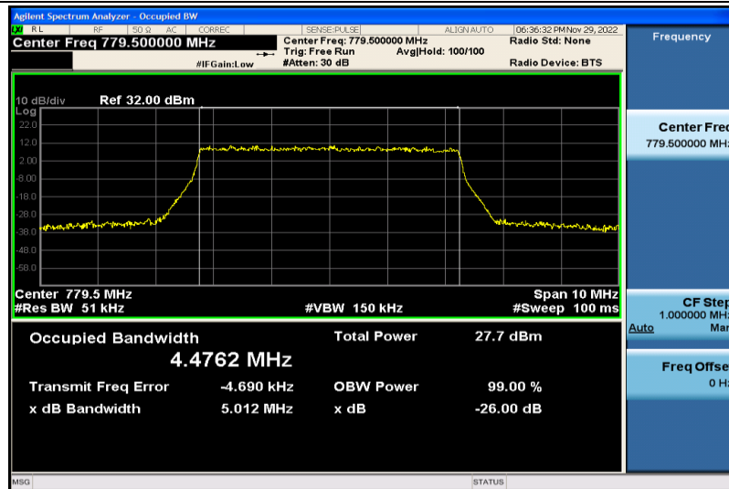
Band13-5MHz-64QAM-23205-25RB#0-4.4762
