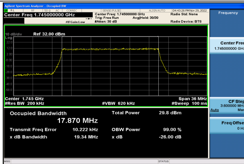
Band66-20MHz-QPSK-132322-100RB#0-17.870
