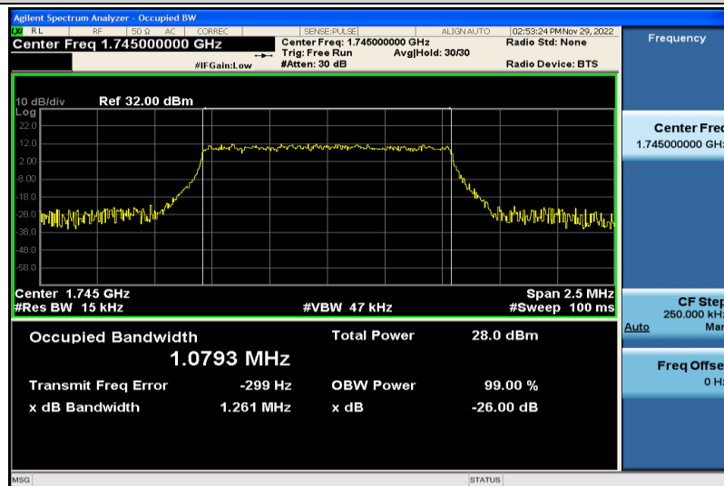
Band66-1.4MHz-QPSK-132322-6RB#0-1.0793
