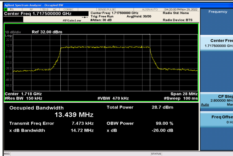
Band66-15MHz-16QAM-132047-75RB#0-13.439
