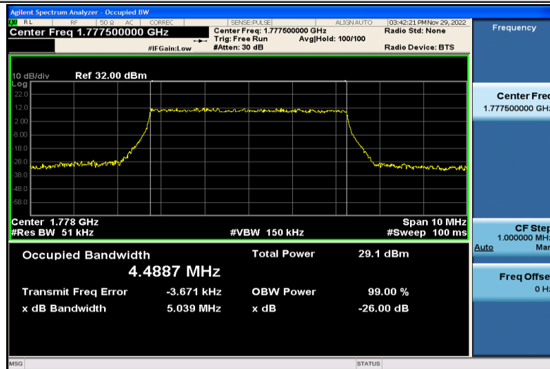
Band66-5MHz-QPSK-132647-25RB#0-4.4887
