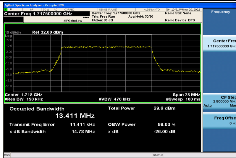
Band66-15MHz-QPSK-132047-75RB#0-13.411
