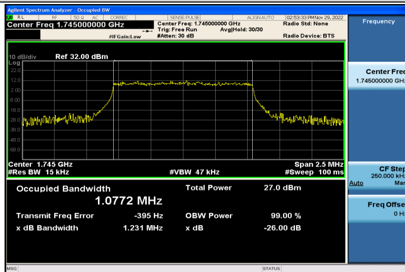
Band66-1.4MHz-16QAM-132322-6RB#0-1.0772
