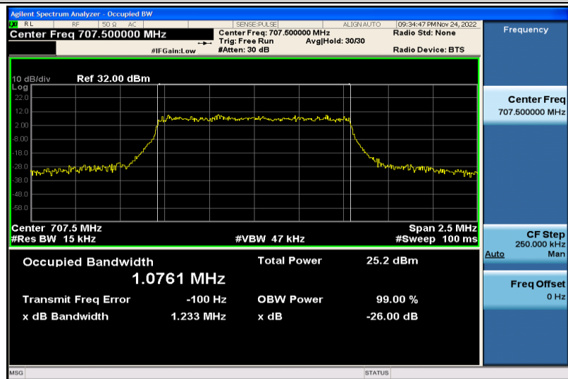
Band12-1.4MHz-16QAM-23095-6RB#0-1.0761
