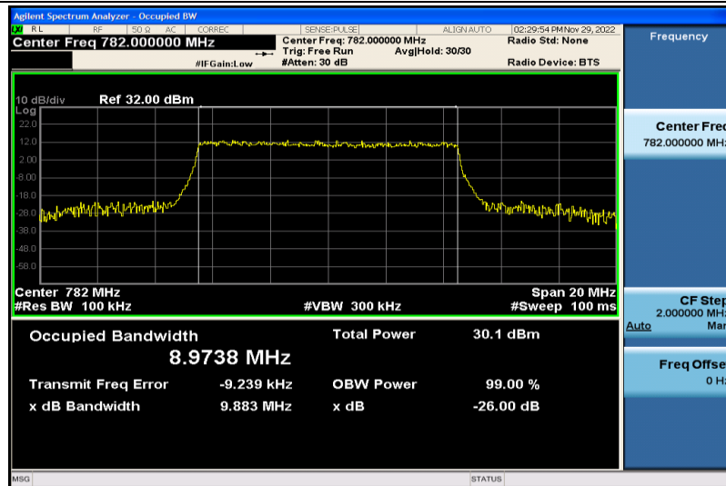
Band13-10MHz-QPSK-23230-50RB#0-8.9738
