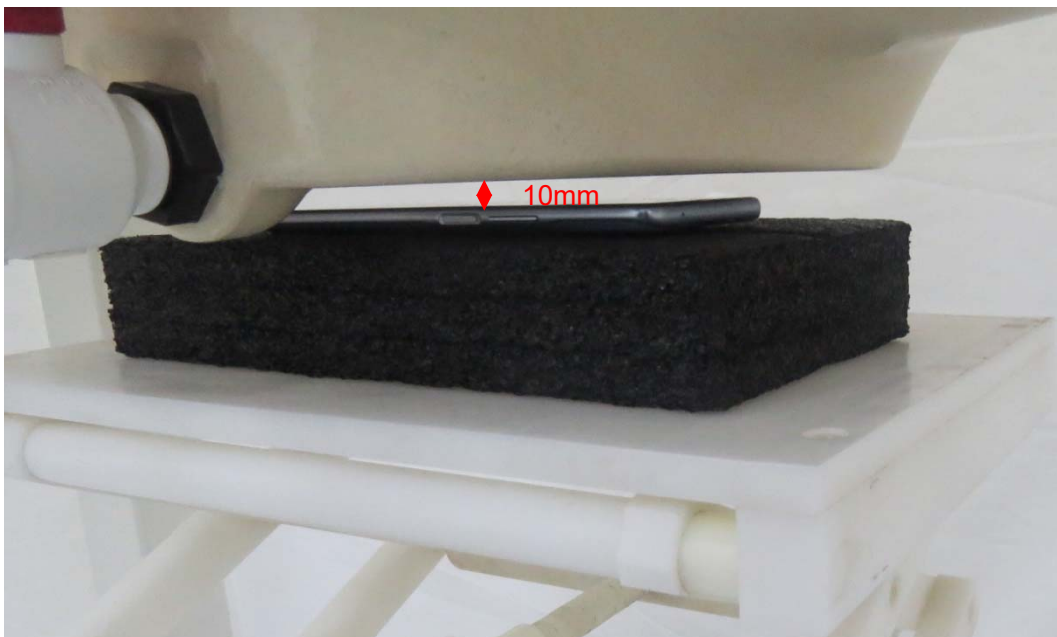
Picture 8: Front Side, the distance from handset to the bottom of the Phantom is 10mm
