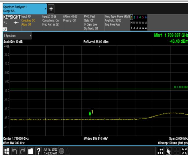
Band66-15MHz-16QAM-132047-1RB#74
