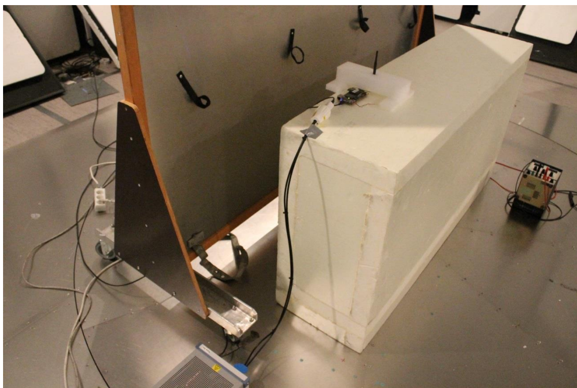
Photograph 6. Conducted Emissions
