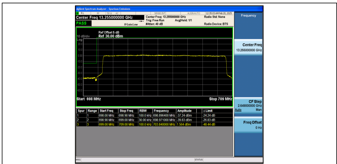
Band12_10MHz_QPSK_23060_50RB#0
