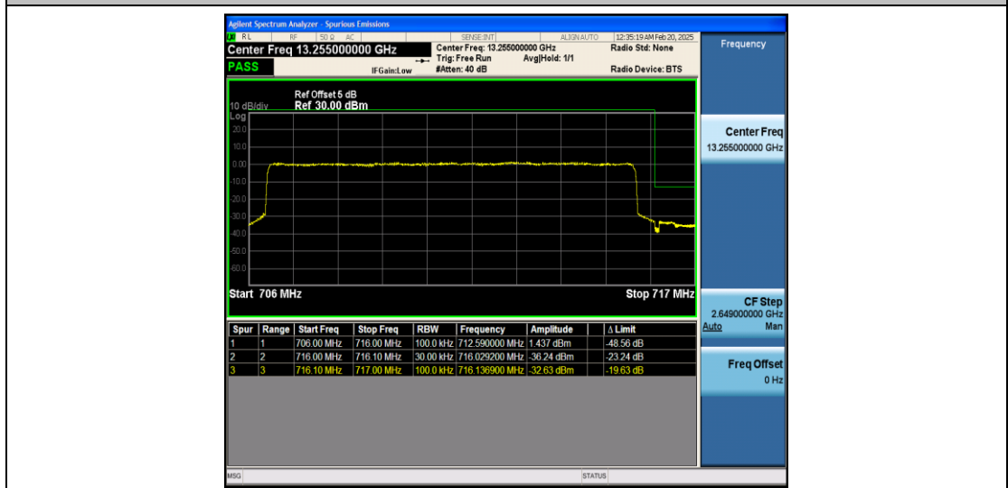
Band12_10MHz_QPSK_23130_50RB#0
