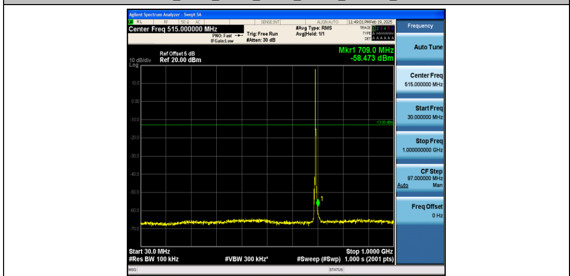
Band12_3MHz_QPSK_23025_1RB#0_30~1000_30~1000
