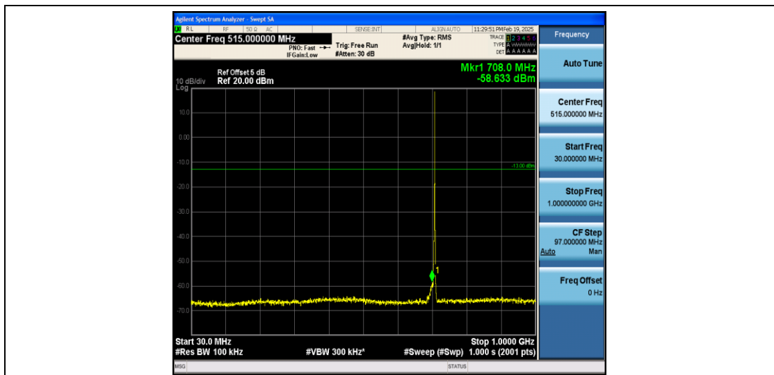
Band12_1.4MHz_16QAM_23173_1RB#0_30~1000_30~1000
