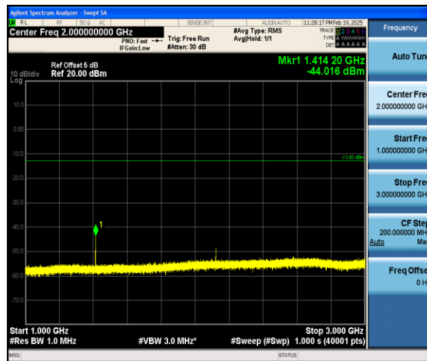
Band12_1.4MHz_16QAM_23095_1RB#0_1000~3000_1000~3000
