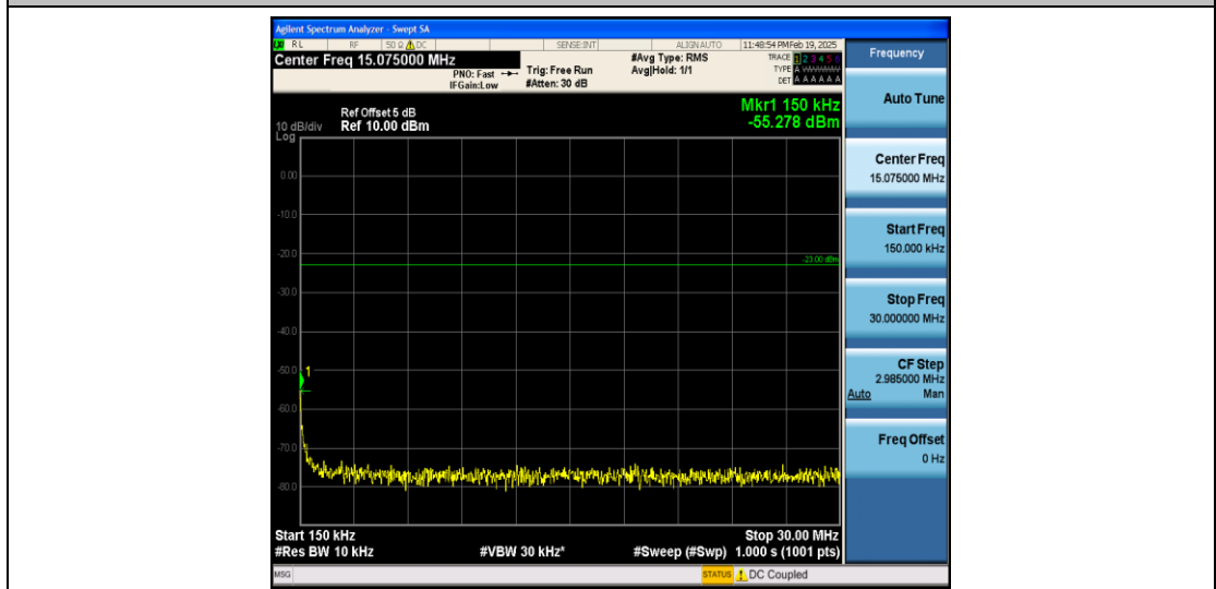
Band12_3MHz_QPSK_23025_1RB#0_0.15~30_0.15~30
