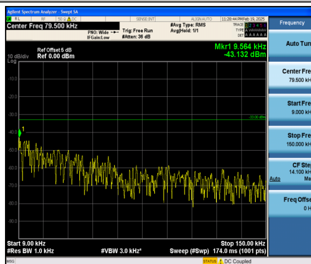
Band12_1.4MHz_QPSK_23173_1RB#0_0.009~0.15_0.009~0.15
