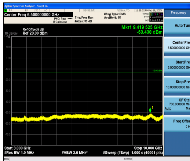
Band12_1.4MHz_16QAM_23095_1RB#0_3000~10000_3000~10000
