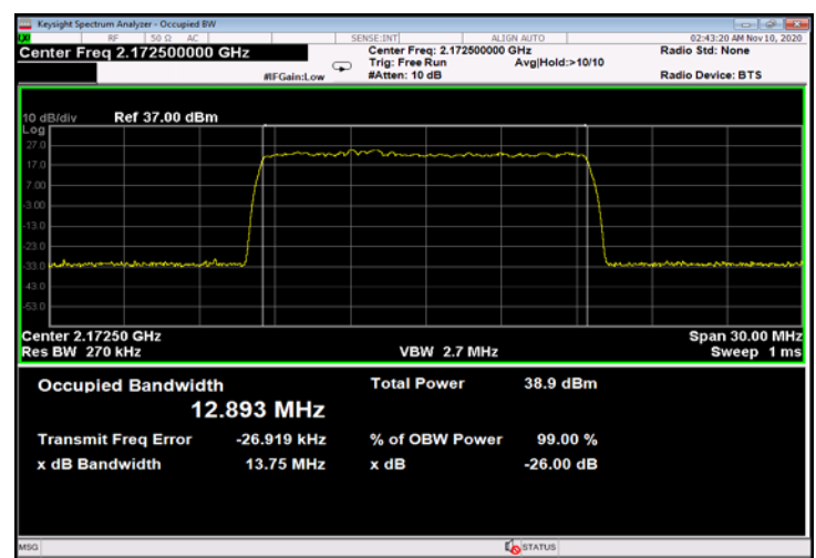
Figure 362: 64QAM 15MHz B.W.; 2172.5MHz, 60kHz - Input
