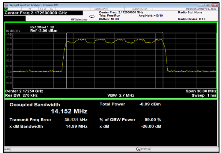
Figure 294: 16QAM 15MHz B.W.; 2172.5MHz, 15kHz - Input
