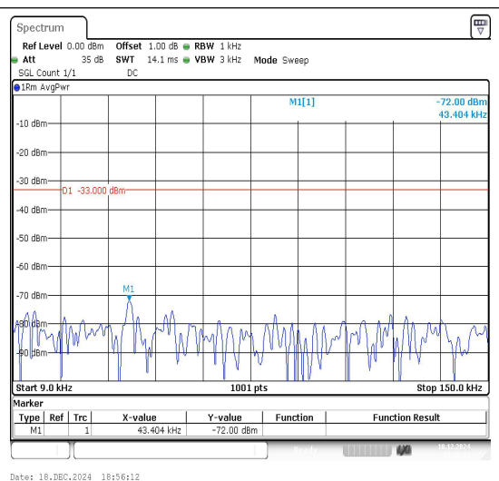
Band13_5MHz_16QAM_23205_1RB#0_0.009~0.15_5_0.009~0.15
