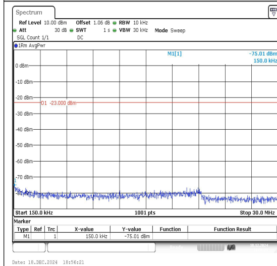
Band13_5MHz_16QAM_23205_1RB#0_0.15~30_0.15~30
