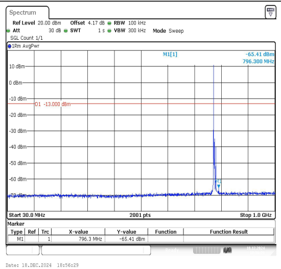
Band13_5MHz_16QAM_23205_1RB#0_30~1000_30~1000
