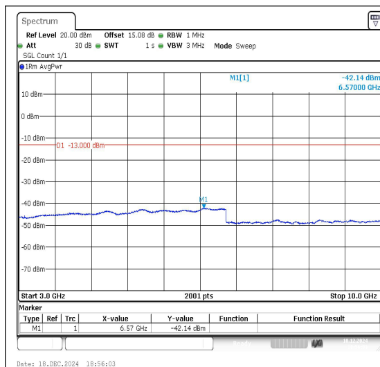
Band13_5MHz_QPSK_23205_1RB#0_3000~10000_00_3000~10000
