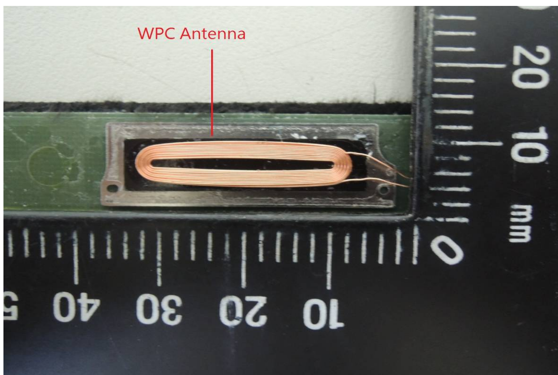
WPC Antenna
