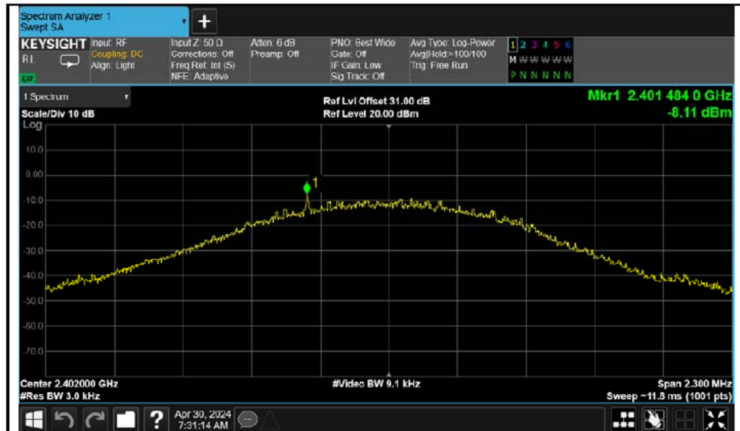
BLE-2402MHz (2Mbps Data Rate)
