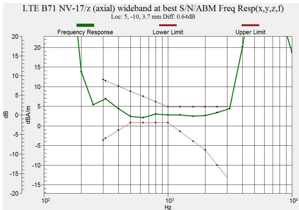
Figure B.41 Frequency Response of LTE Band 71 Ant.2 (Google Duo)
