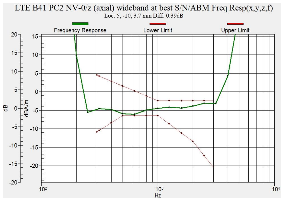
Figure B.40 Frequency Response of LTE Band 41 PC2 Ant.2 (Google Duo)
