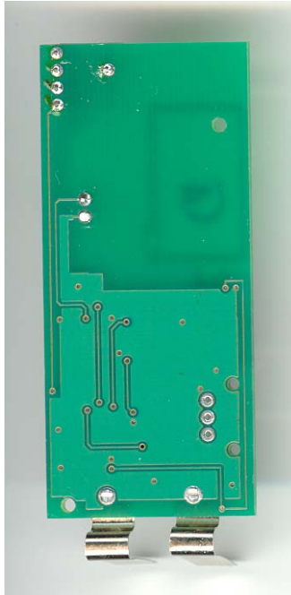
Photo 4. Internal View, Bottom Side
