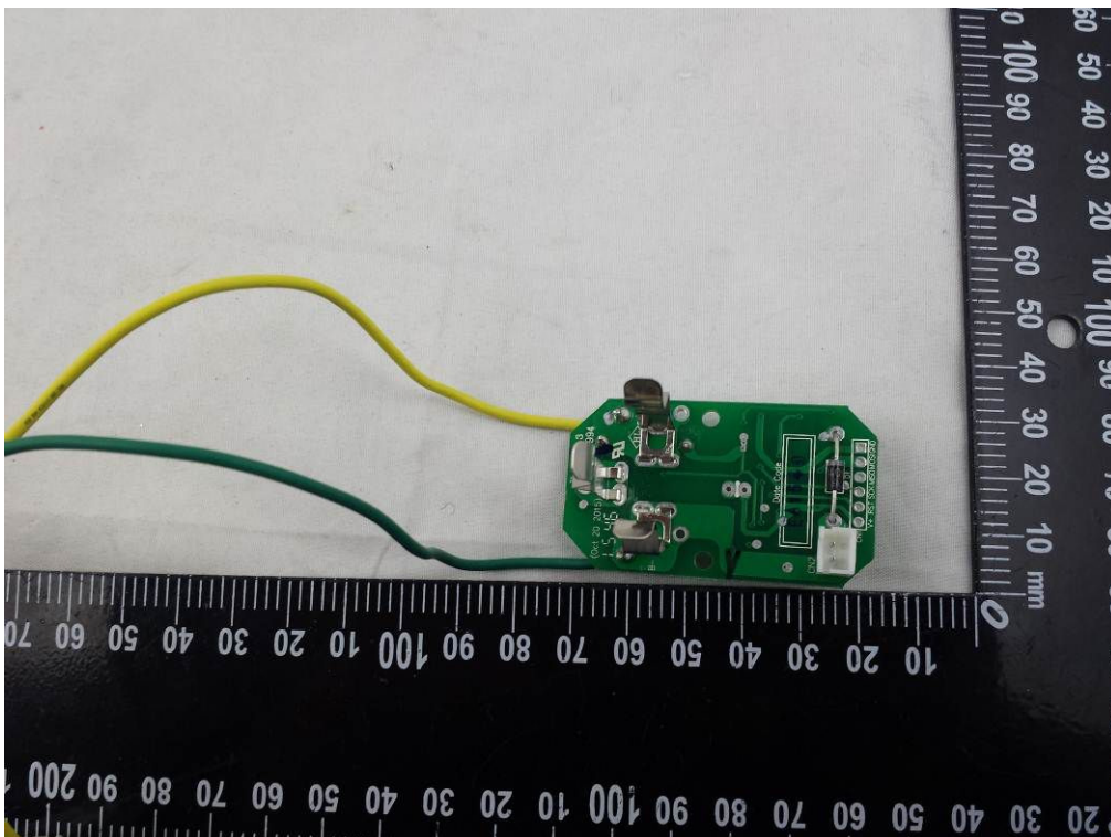
Board (Rear)
