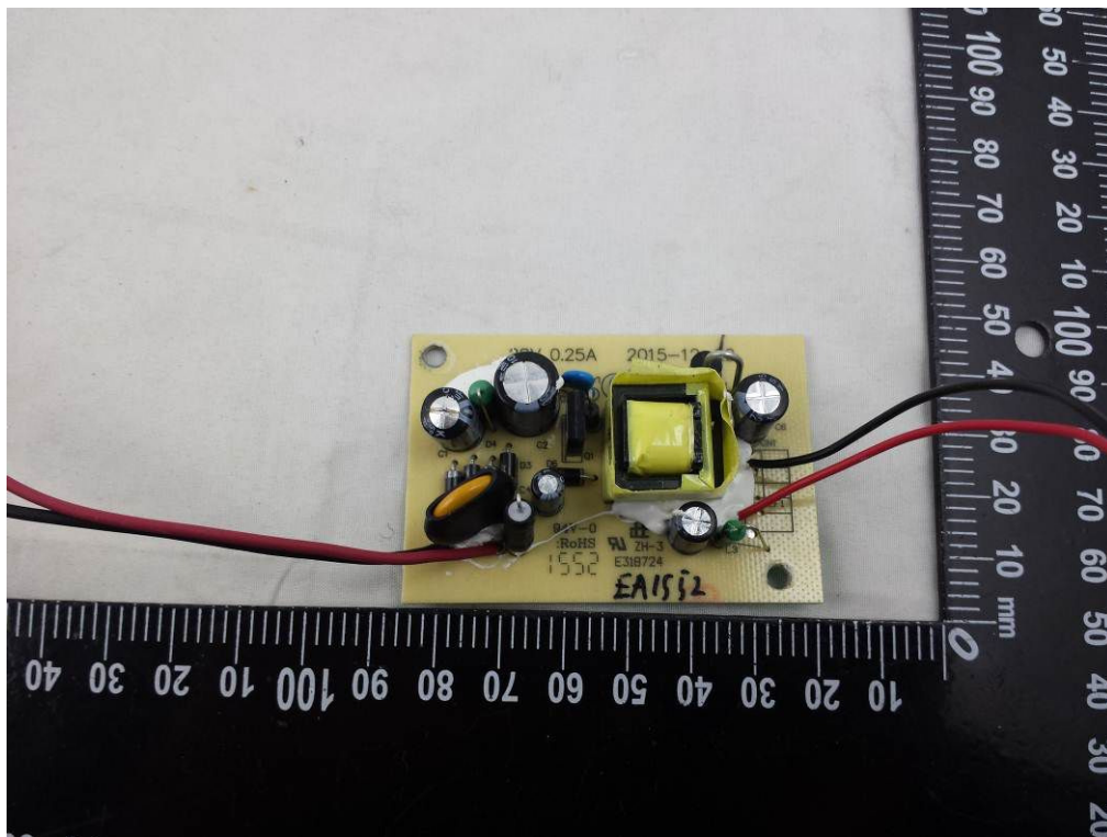
Board (Front)
