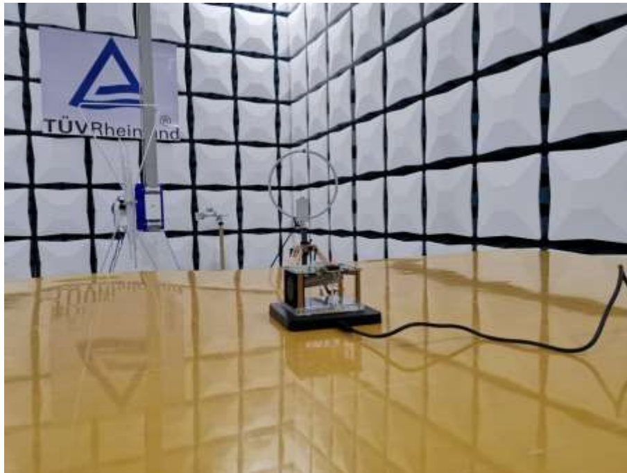
Photograph 1: Set-up photo for Radiated Emission, 9KHz - 30MHz
