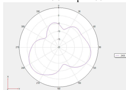
Theta =90 freq=2400MHz
