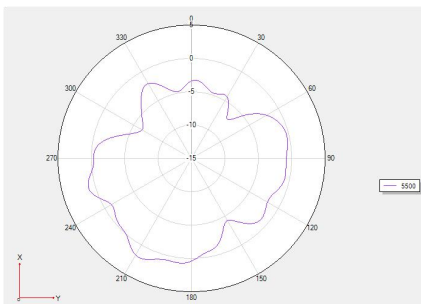
Theta =90 freq=5500MHz
