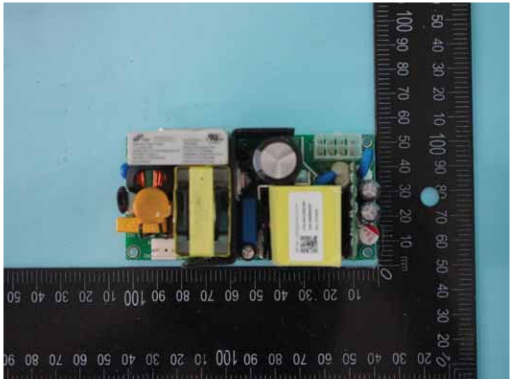
Switching Power Supply 1 (Specify 2 qty)
