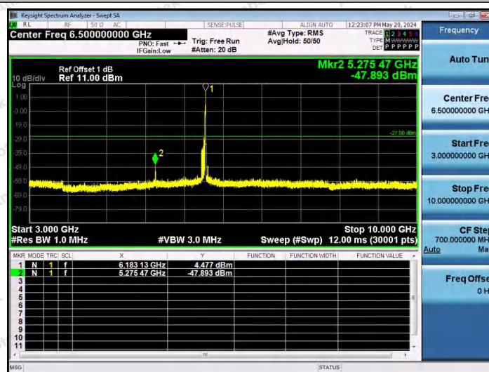
11AX80SISO-Ant1-6145-26Tone-RU36-3000~10000-PASS
