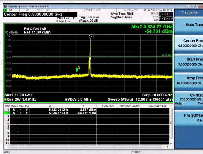
11AX80SISO-Ant1-6385-26Tone-RU36-3000~10000-PASS
