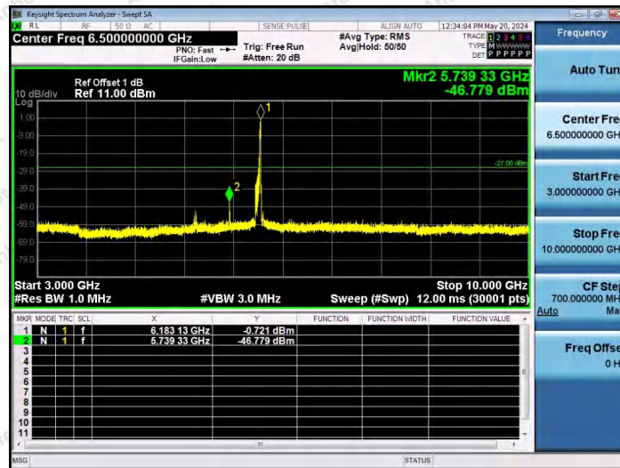
11AX80SISO-Ant1-6145-106Tone-RU60-3000~10000-PASS
