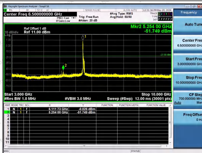
11AX80SISO-Ant1-6145-106Tone-RU53-3000~10000-PASS
