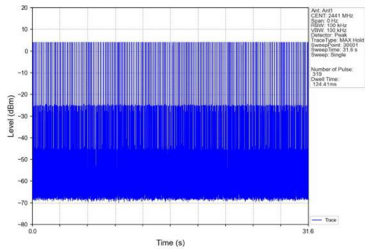
Dwell_Time_(Hopping)_NVNT_ANT1_3-DH1_2441_Accumulated
