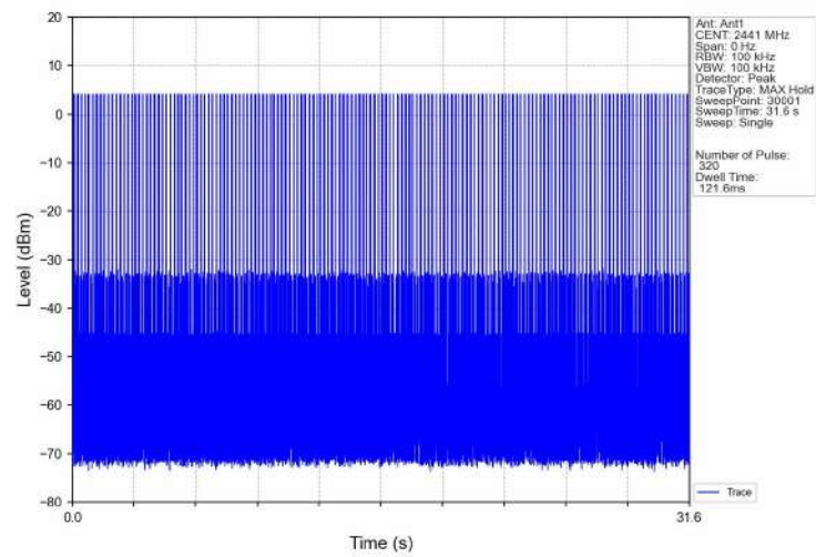
Dwell_Time_(Hopping)_NVNT_ANT1_1-DH1_2441_Accumulated
