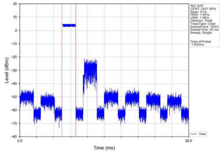
Dwell_Time_(Hopping)_NVNT_ANT1_3-DH3_2441_Accumulated
