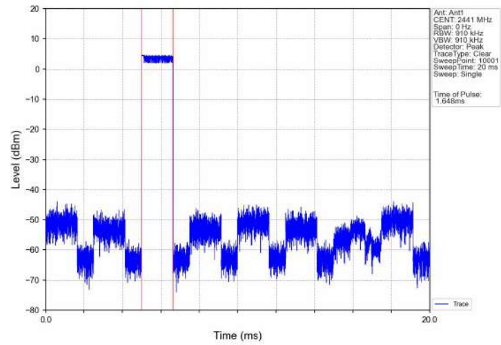
Dwell_Time_(Hopping)_NVNT_ANT1_2-DH3_2441_Accumulated
