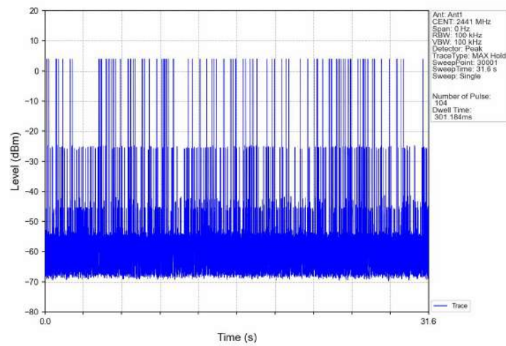
Dwell_Time_(Hopping)_NVNT_ANT1_2-DH5_2441_Accumulated
