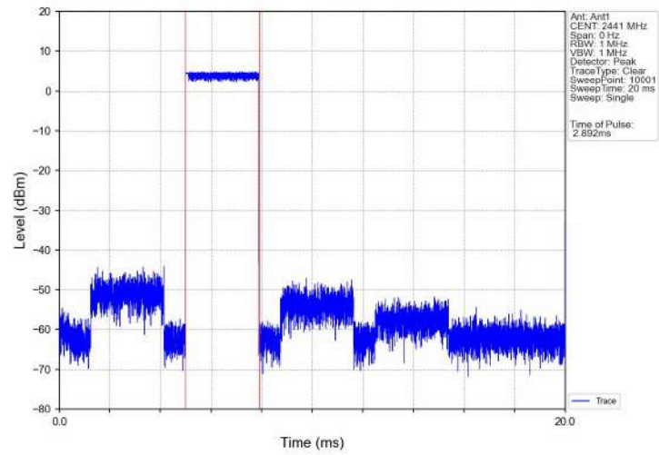
Dwell_Time_(Hopping)_NVNT_ANT1_3-DH5_2441_Accumulated
