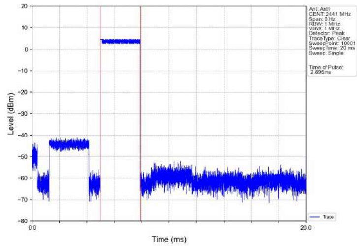
Dwell_Time_(Hopping)_NVNT_ANT1_2-DH5_2441_Accumulated
