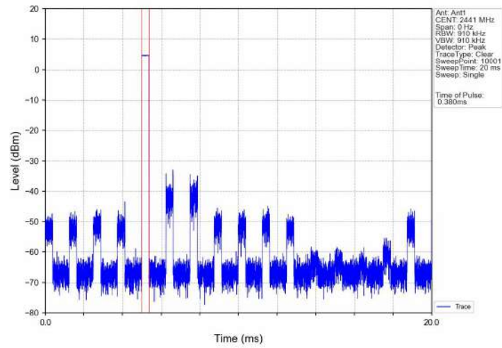
Dwell_Time_(Hopping)_NVNT_ANT1_1-DH1_2441_Accumulated
