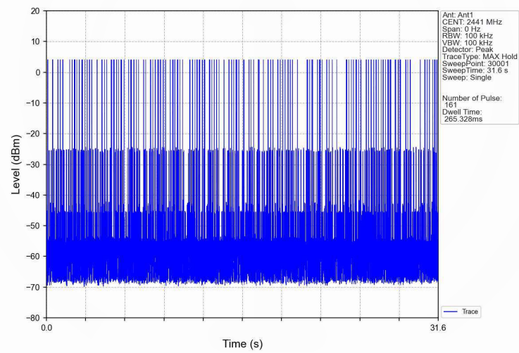
Dwell_Time_(Hopping)_NVNT_ANT1_2-DH3_2441_Accumulated
