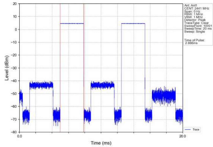
Dwell_Time_(Hopping)_NVNT_ANT1_DH5_2441_Accumulated
