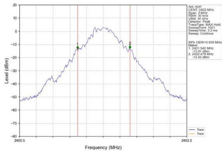
99%_Occupied_Bandwidth_NVNT_ANT1_DH5_2402
