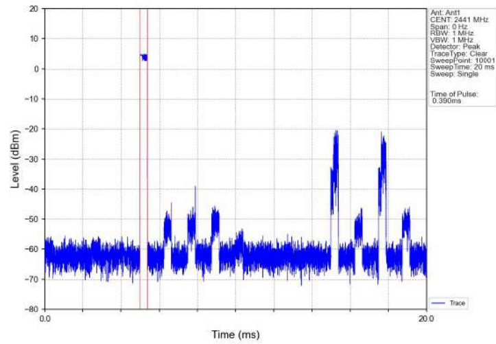
Dwell_Time_(Hopping)_NVNT_ANT1_3-DH1_2441_Accumulated
