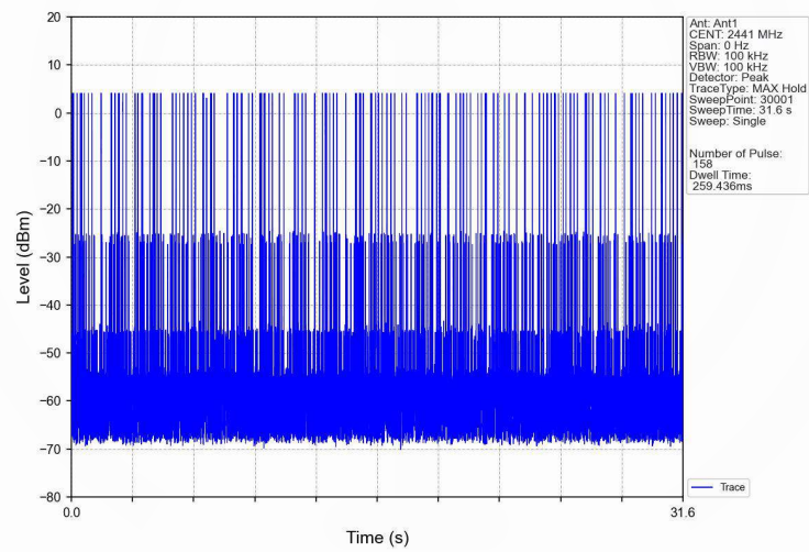
Dwell_Time_(Hopping)_NVNT_ANT1_3-DH3_2441_Accumulated
