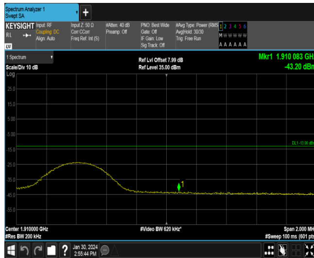
Band2-10MHz-16QAM-19150-1RB#49
