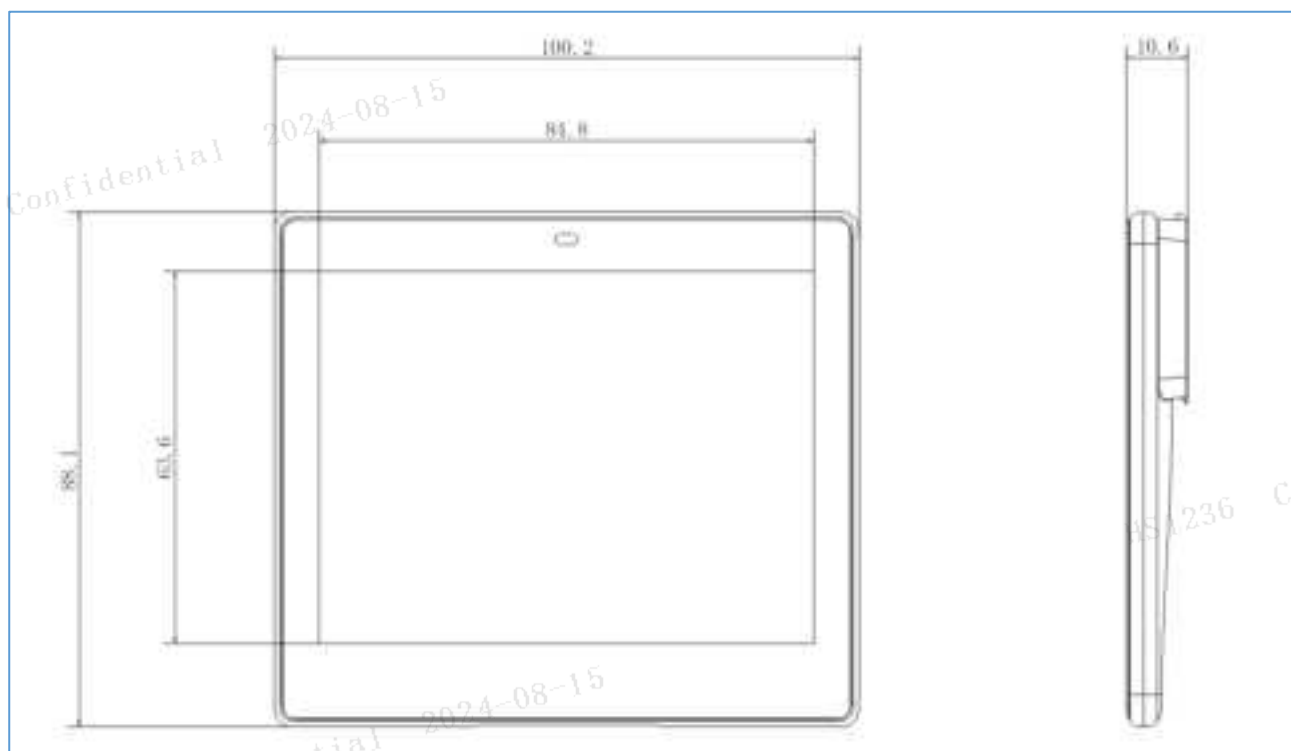
Figure 2-9 4.2" dimensions
