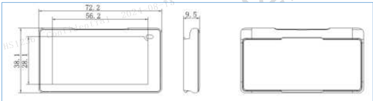
Figure 2-6 2.6" dimensions
