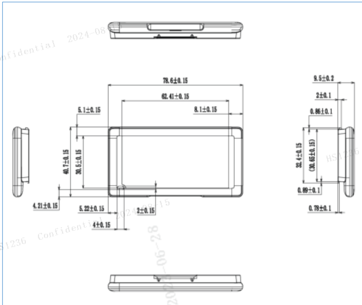
Figure 2-7 2.8" dimensions
