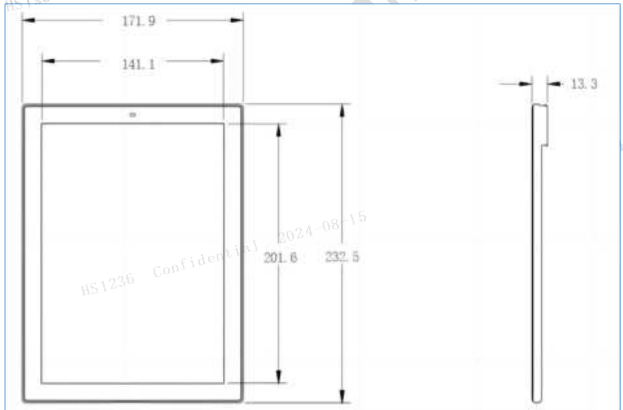
Figure 2-12 9.7" dimensions
