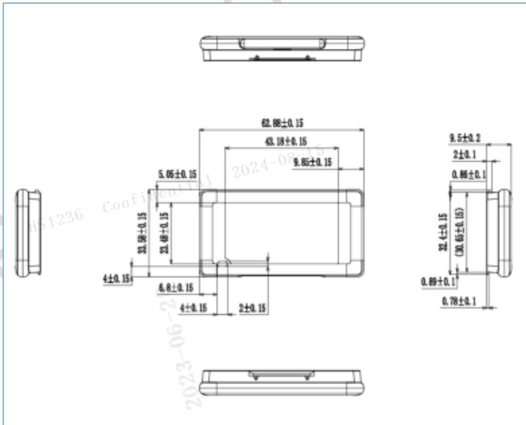
Figure 2-4 2.0" dimensions
