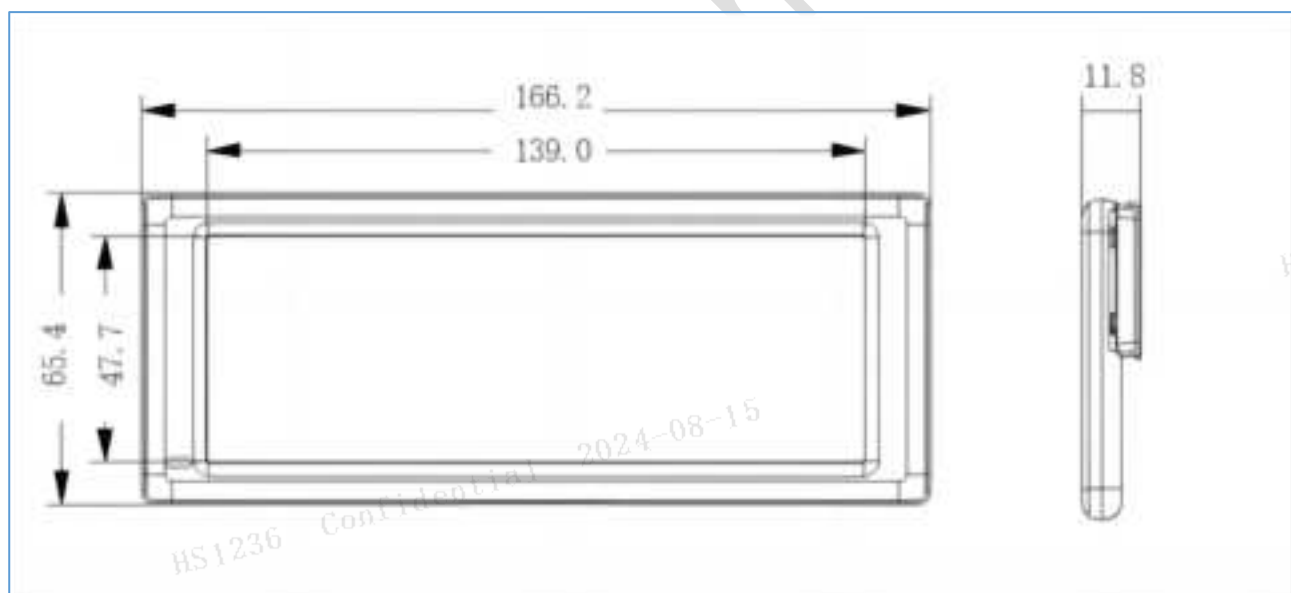
Figure 2-10 5.9" dimensions
