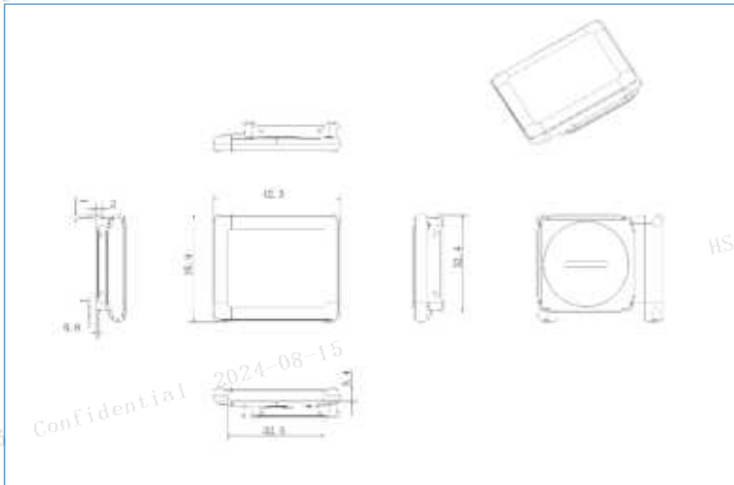
Figure 2-3 1.6" dimensions
