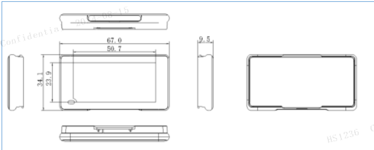
Figure 2-5 2.3" dimensions
