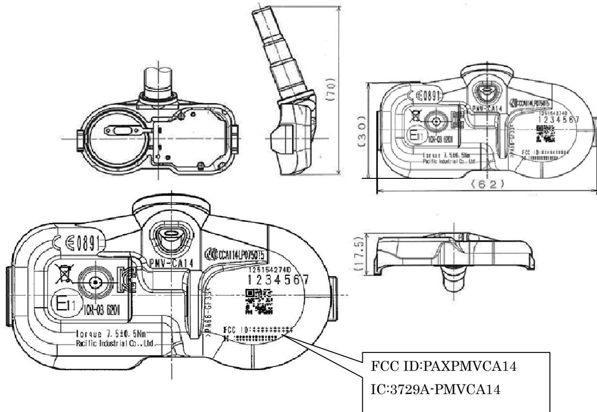
Fig 5. Marking location and dimension
