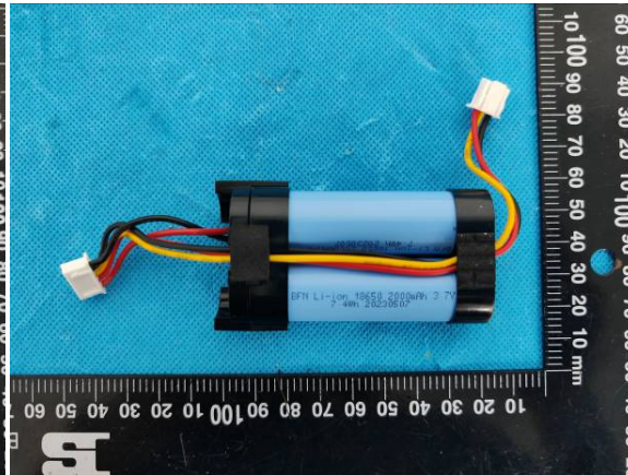
battery
