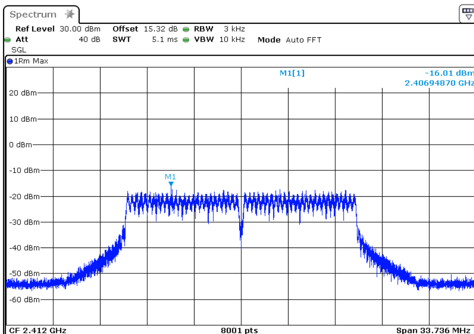
802.11g Channel Low 2412MHz
