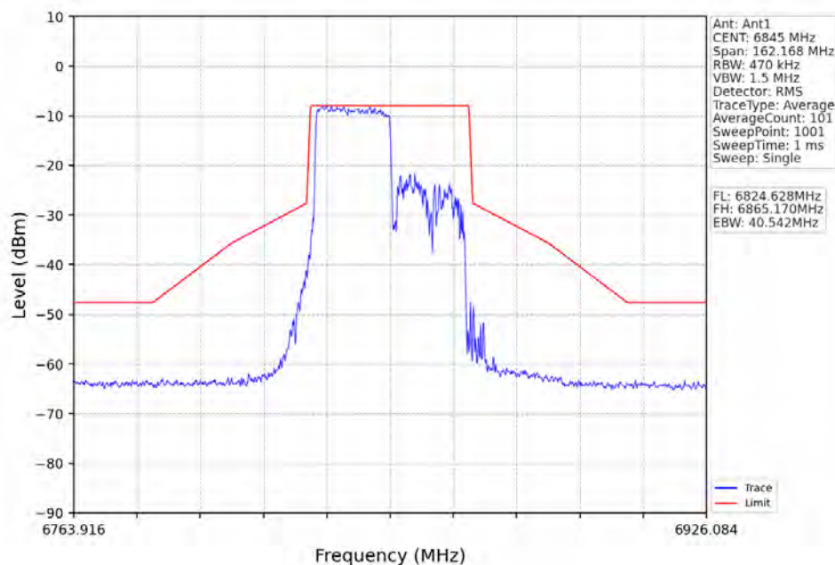
802.11ax(HEW40)_HCH_6845MHz_RU242_Left_Ant1_NTNV
