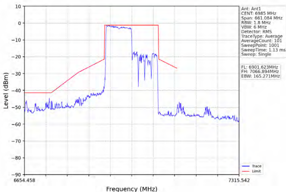
802.11ax(HEW160)_MCH_6985MHz_RU996_Right_Ant1_NTNV
