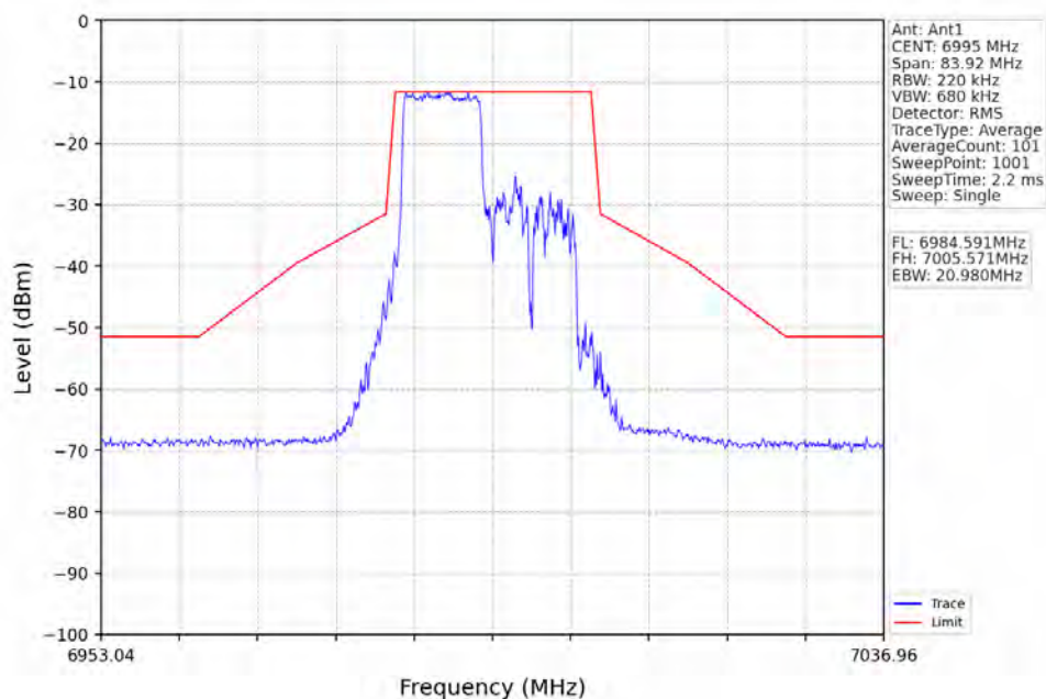
802.11ax(HEW20)_MCH_6995MHz_RU106_Left_Ant1_NTNV
