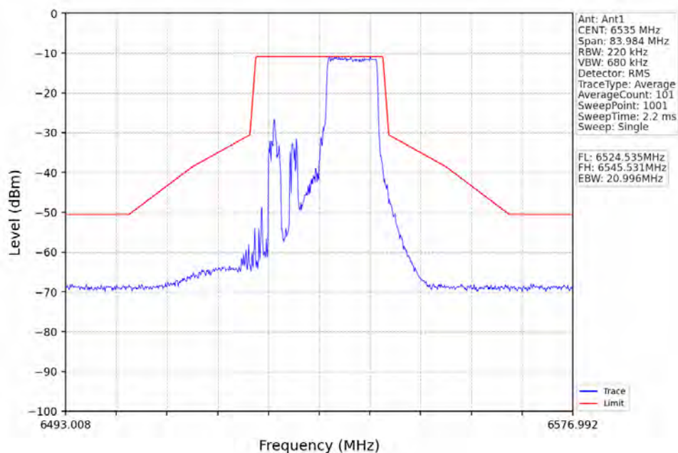
802.11ax(HEW20)_LCH_6535MHz_RU106_Right_Ant1_NTNV
