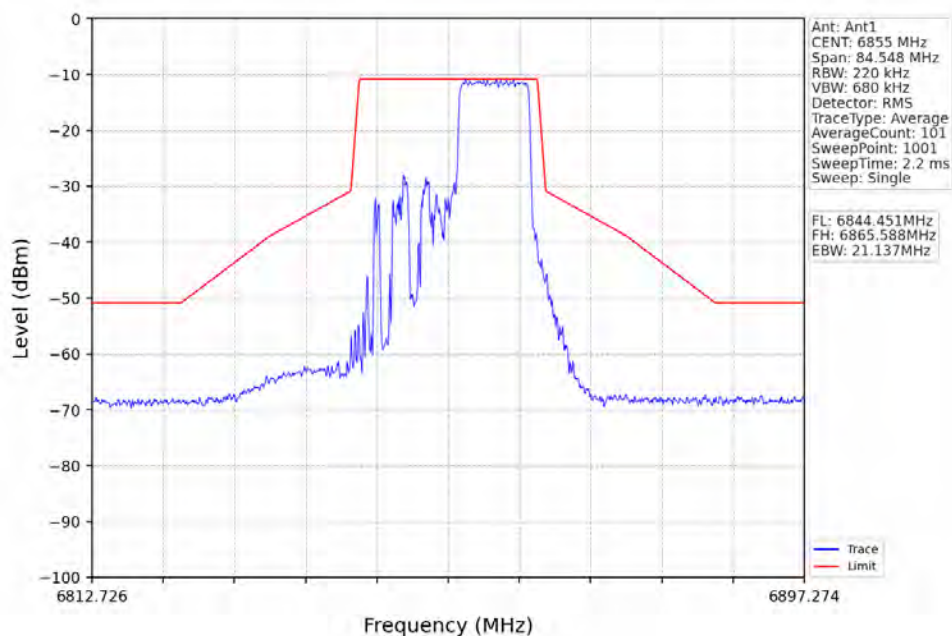
802.11ax(HEW20)_HCH_6855MHz_RU106_Right_Ant1_NTNV
