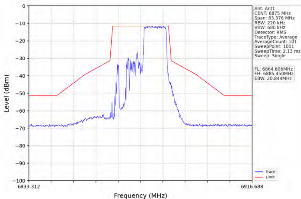
802.11ax(HEW20)_HCH_6875MHz_RU106_Right_Ant1_NTNV
