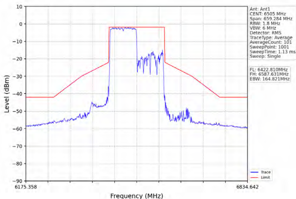
802.11ax(HEW160)_HCH_6505MHz_RU996_Right_Ant1_NTNV
