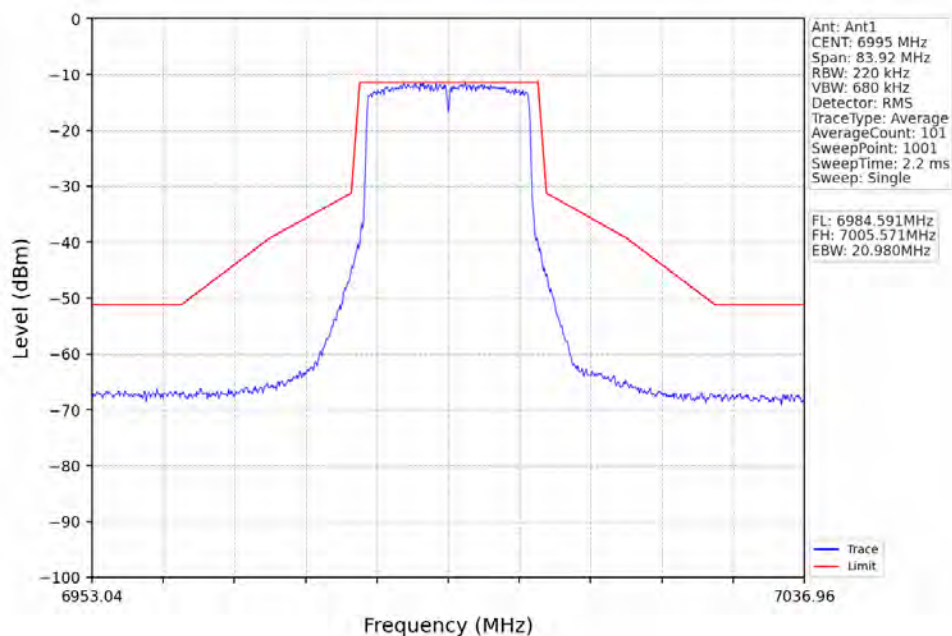
802.11ax(HEW20)_MCH_6995MHz_RU242_Left_Ant1_NTNV
