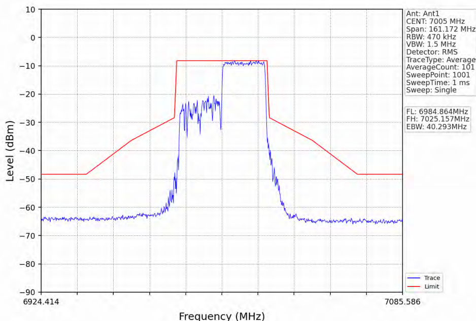
802.11ax(HEW40)_MCH_7005MHz_RU242_Right_Ant1_NTNV
