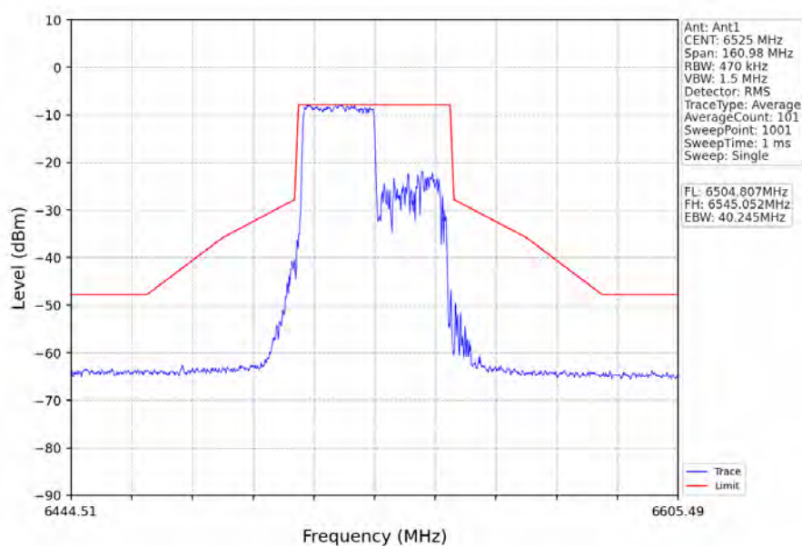
802.11ax(HEW40)_HCH_6525MHz_RU242_Right_Ant1_NTNV
