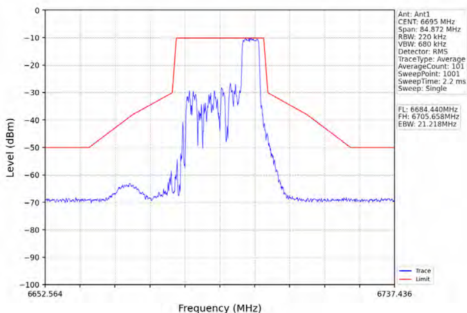
802.11ax(HEW20)_MCH_6695MHz_RU106_Left_Ant1_NTNV
