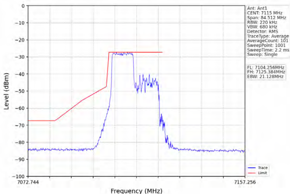
802.11ax(HEW20)_HCH_7115MHz_RU106_Right_Ant1_NTNV
