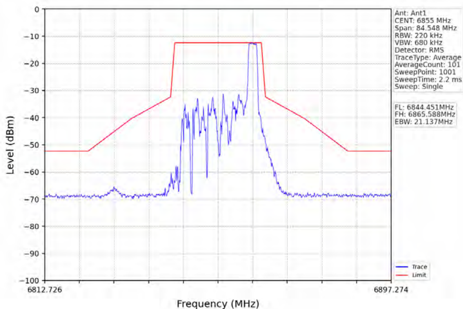
802.11ax(HEW20)_HCH_6855MHz_RU26_Right_Ant1_NTNV
