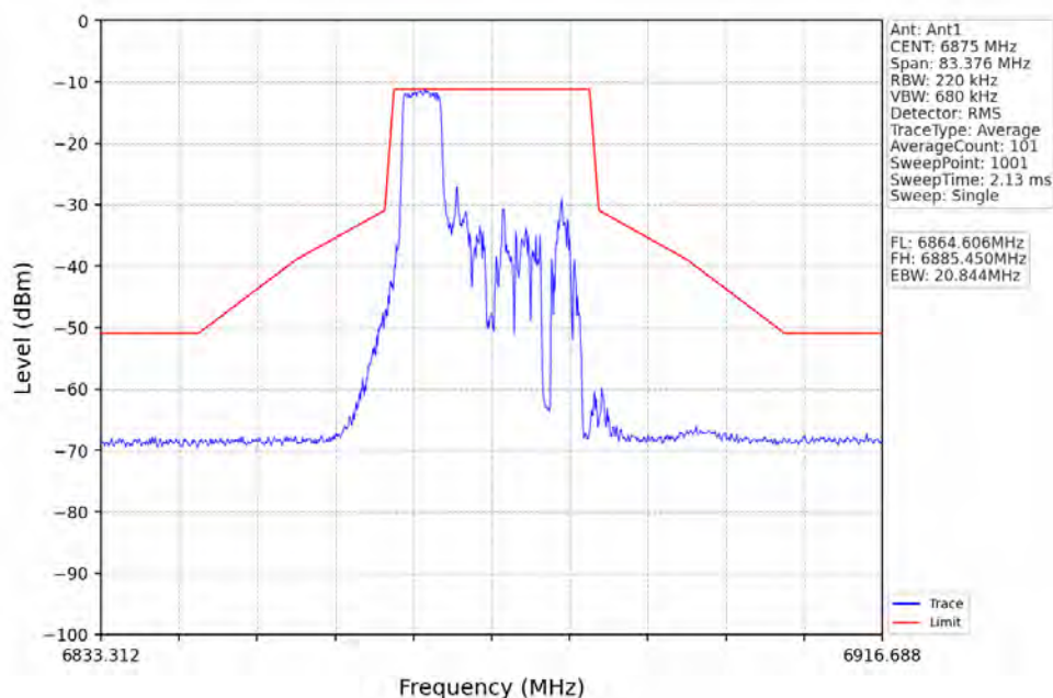
802.11ax(HEW20)_HCH_6875MHz_RU52_Right_Ant1_NTNV
