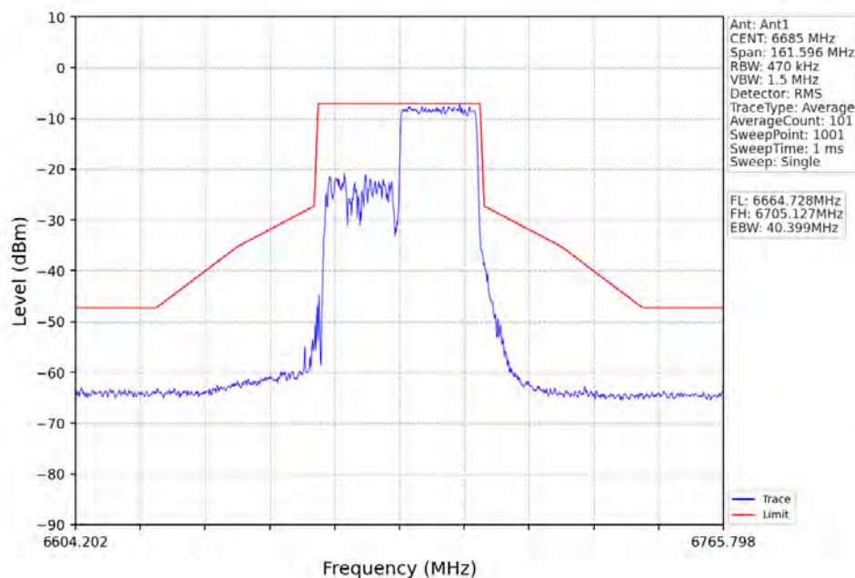
802.11ax(HEW40)_MCH_6685MHz_RU242_Right_Ant1_NTNV
