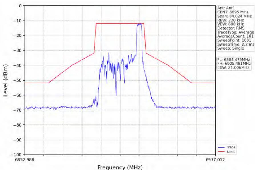
802.11ax(HEW20)_LCH_6895MHz_RU26_Right_Ant1_NTNV
