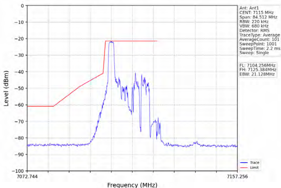
802.11ax(HEW20)_HCH_7115MHz_RU26_Right_Ant1_NTNV
