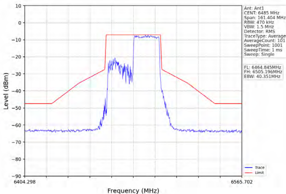
802.11ax(HEW40)_MCH_6485MHz_RU242_Right_Ant1_NTNV
