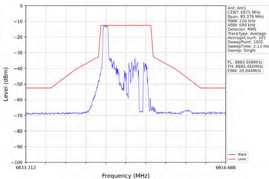
802.11ax(HEW20)_HCH_6875MHz_RU26_Right_Ant1_NTNV
