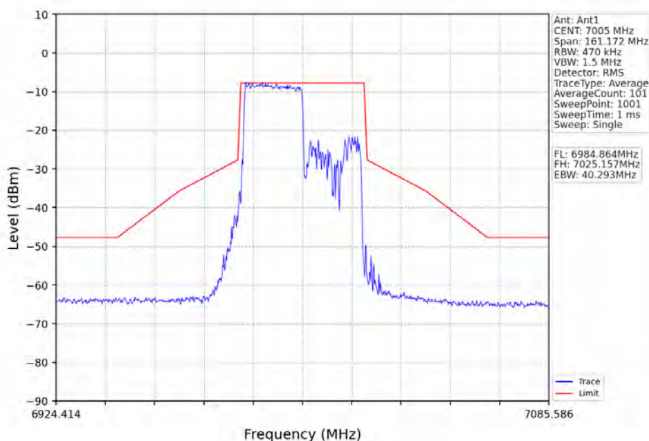
802.11ax(HEW40)_MCH_7005MHz_RU242_Right_Ant1_NTNV
