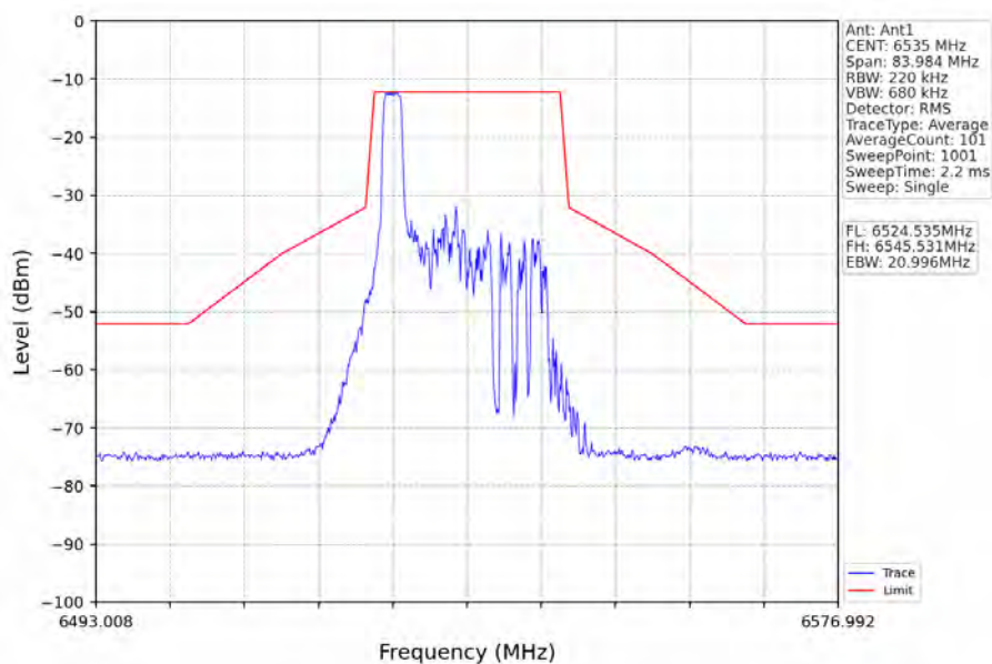
802.11ax(HEW20)_LCH_6535MHz_RU26_Right_Ant1_NTNV
