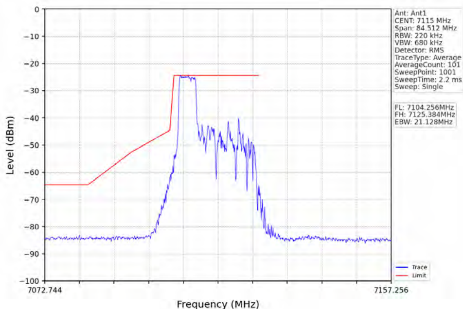
802.11ax(HEW20)_HCH_7115MHz_RU52_Right_Ant1_NTNV
