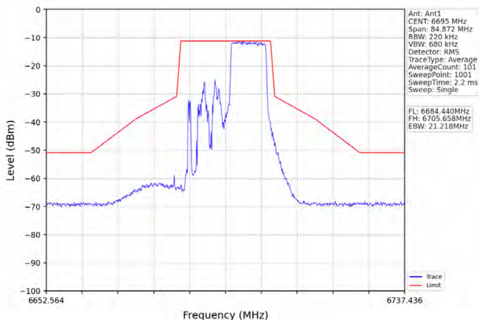
802.11ax(HEW20)_MCH_6695MHz_RU242_Left_Ant1_NTNV
