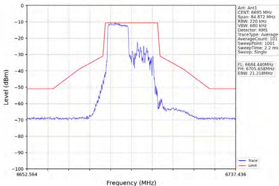
802.11ax(HEW20)_MCH_6695MHz_RU106_Left_Ant1_NTNV
