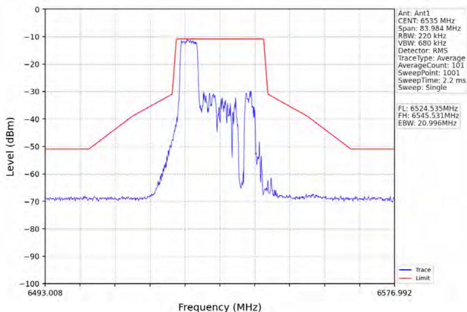
802.11ax(HEW20)_LCH_6535MHz_RU52_Right_Ant1_NTNV
