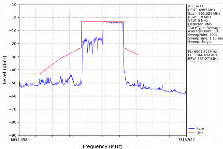
802.11ax(HEW160)_MCH_6985MHz_RU996_Right_Ant1_NTNV
