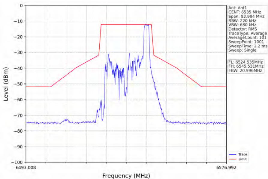
802.11ax(HEW20)_LCH_6535MHz_RU26_Right_Ant1_NTNV
