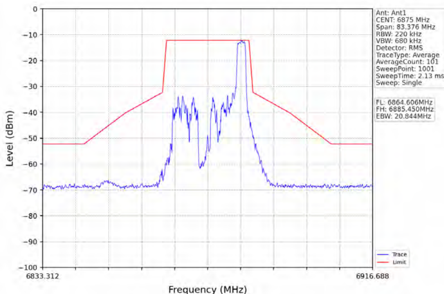
802.11ax(HEW20)_HCH_6875MHz_RU26_Right_Ant1_NTNV
