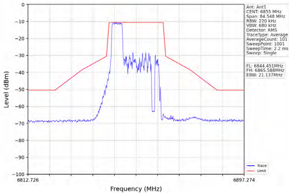
802.11ax(HEW20)_HCH_6855MHz_RU52_Right_Ant1_NTNV
