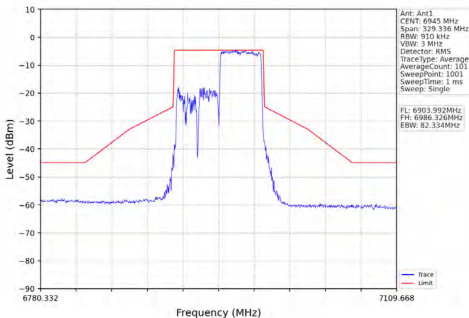
802.11ax(HEW80)_LCH_6945MHz_RU484_Right_Ant1_NTNV
