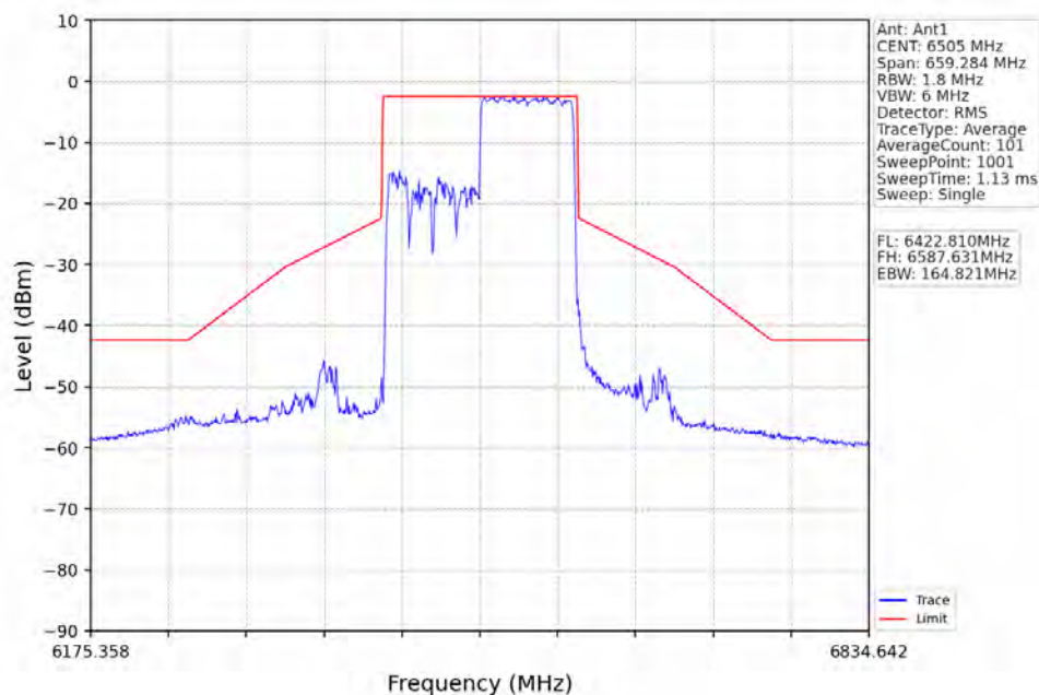
802.11ax(HEW160)_HCH_6505MHz_RU996_Right_Ant1_NTNV
