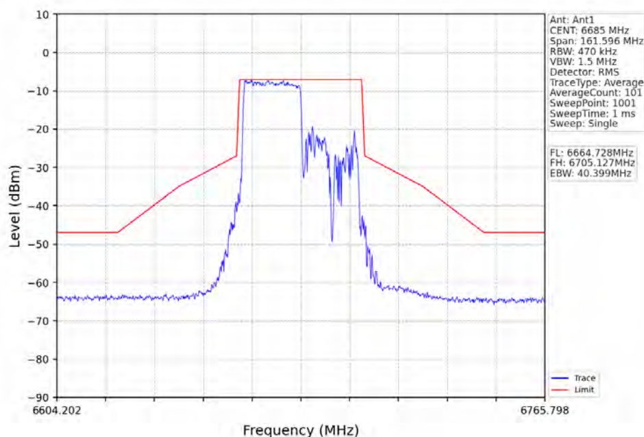
802.11ax(HEW40)_MCH_6685MHz_RU242_Right_Ant1_NTNV
