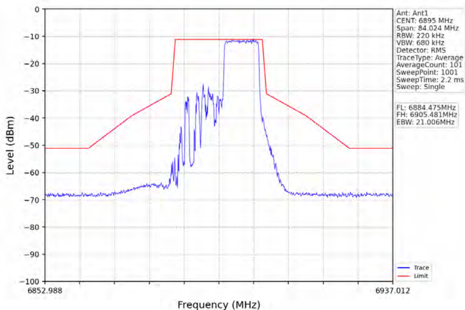
802.11ax(HEW20)_LCH_6895MHz_RU106_Right_Ant1_NTNV
