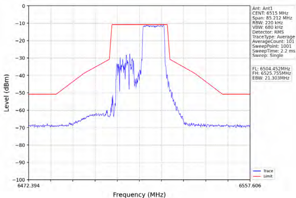
802.11ax(HEW20)_HCH_6515MHz_RU106_Right_Ant1_NTNV
