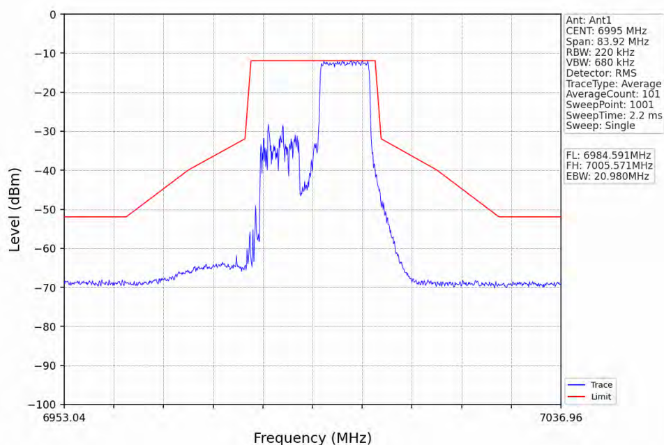
802.11ax(HEW20)_MCH_6995MHz_RU242_Left_Ant1_NTNV
