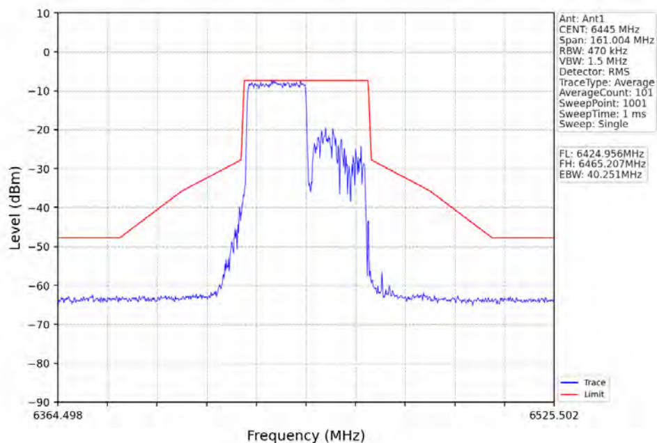
802.11ax(HEW40)_LCH_6445MHz_RU242_Left_Ant1_NTNV
