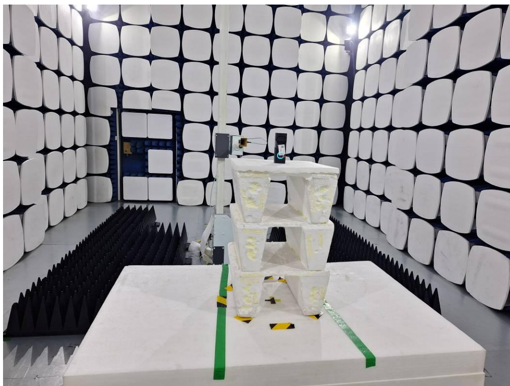
Above 18 GHz Type-C port
