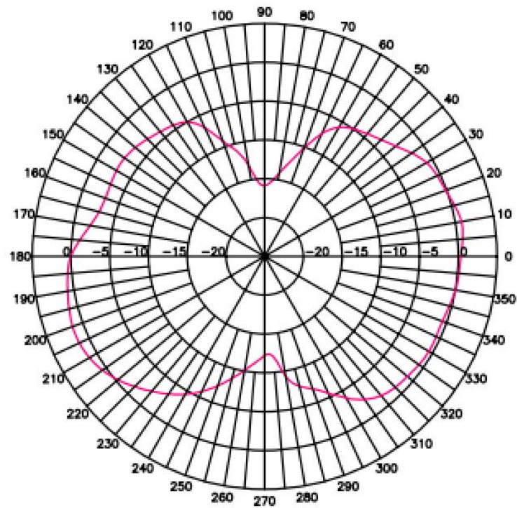
E-Plane Pattern @ 2.45GHz
