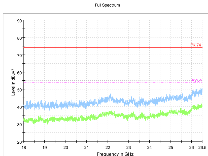
Pic7. Radiated emission (18GHz – 26GHz)
