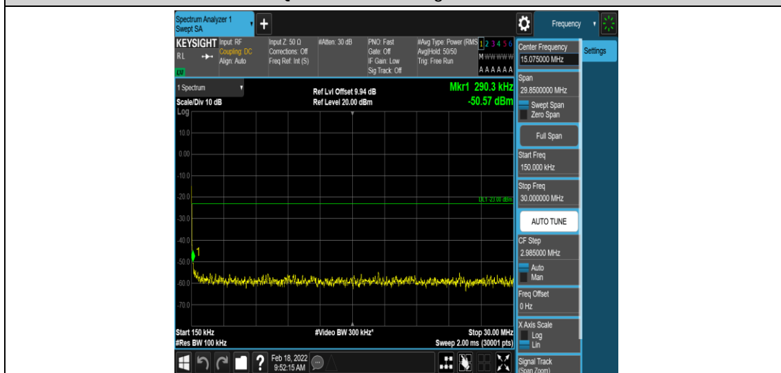
Band2-20MHz-16QAM-19100-1-0-High-0.15-30--50.57-PASS
