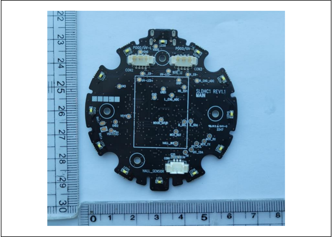
CRADLE Main Board Front
