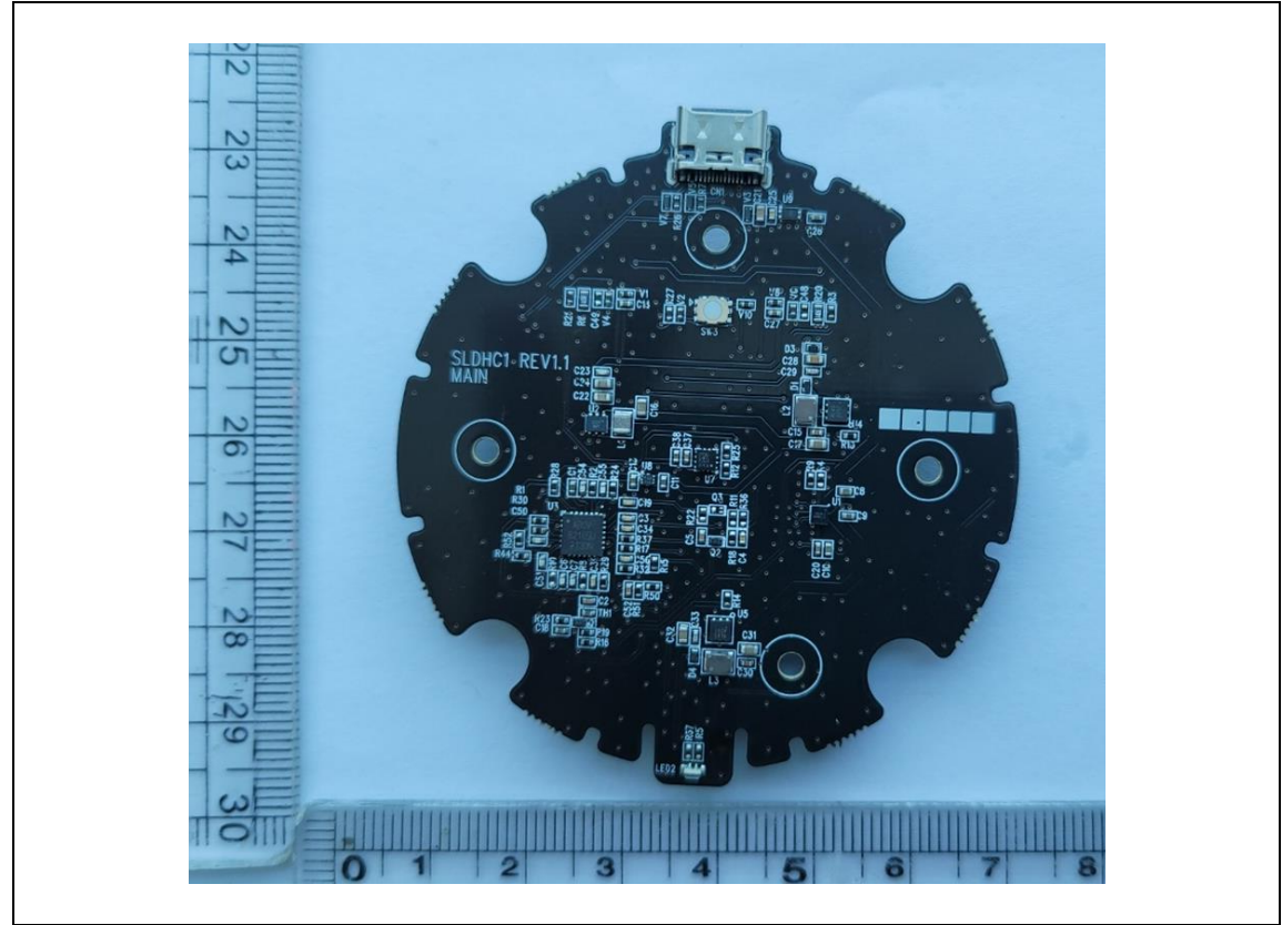
CRADLE Main Board Rear
