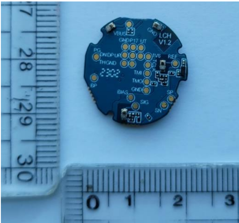
LEFT Main Board Rear
