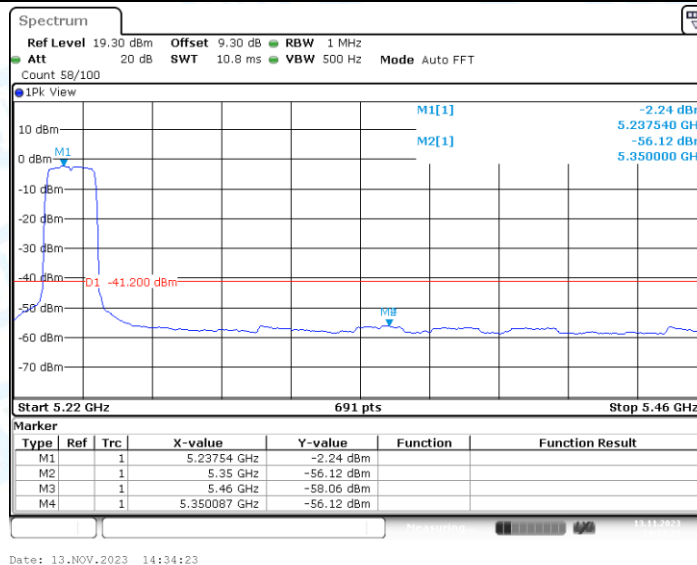
11A_Ant2_High_5240_Peak
