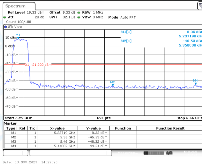
11A_Ant2_High_5240_AV
