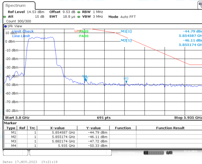
11AC20MIMO_Ant2_High_5825
