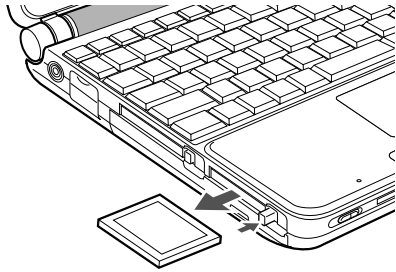
Figure 4-12 Removing a CF Card
