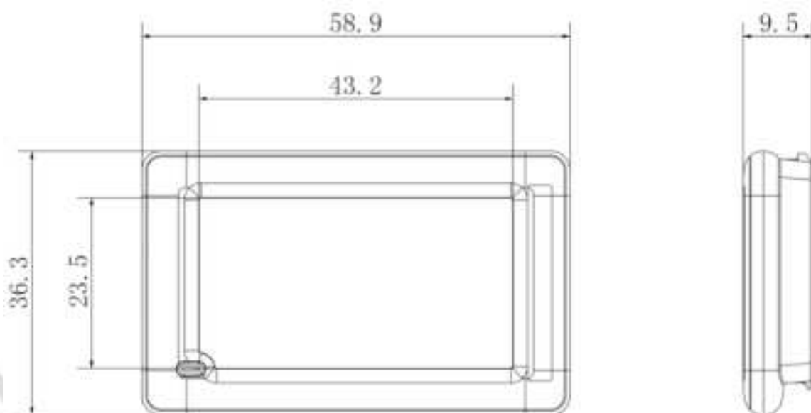
Figure 2-4 2.0" dimension
