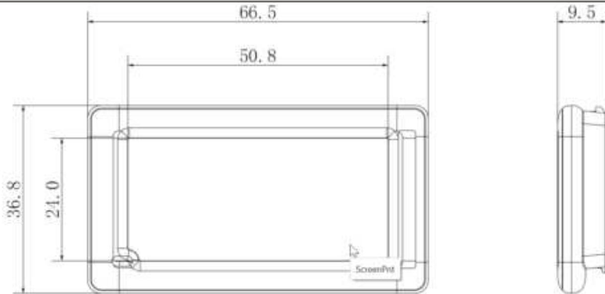
Figure 2-5 2.3' dimension
