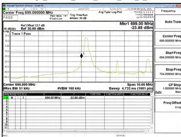
Band Edge_Band12_5MHz_QPSK_RB1_0_CH23035
