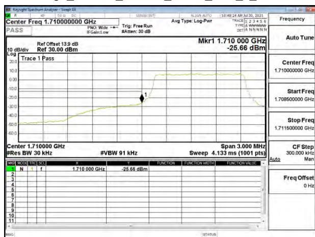
Band Edge_Band66_1.4MHz_QPSK_RB6_0_CH131979
