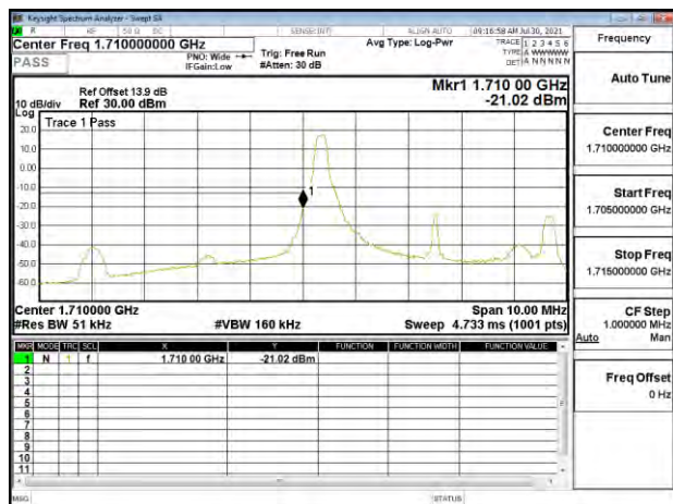
Band Edge_Band4_5MHz_QPSK_RB1_0_CH19975
