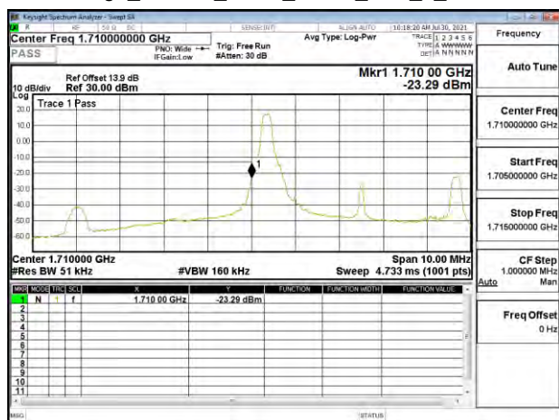
Band Edge_Band66_5MHz_QPSK_RB1_0_CH131997
