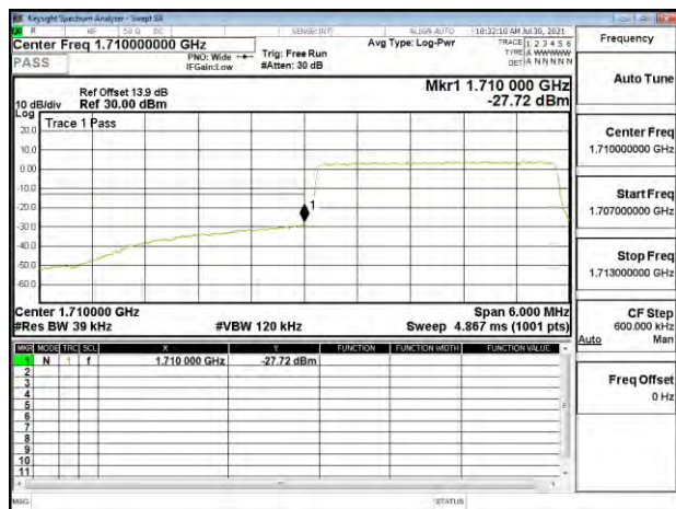
Band Edge_Band66_3MHz_QPSK_RB15_0_CH131987
