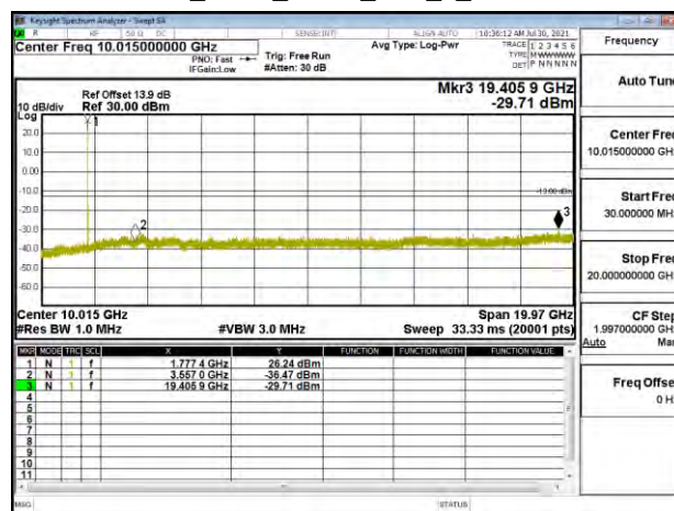
Band66_3MHz_QPSK_RB1_0_CH132657
