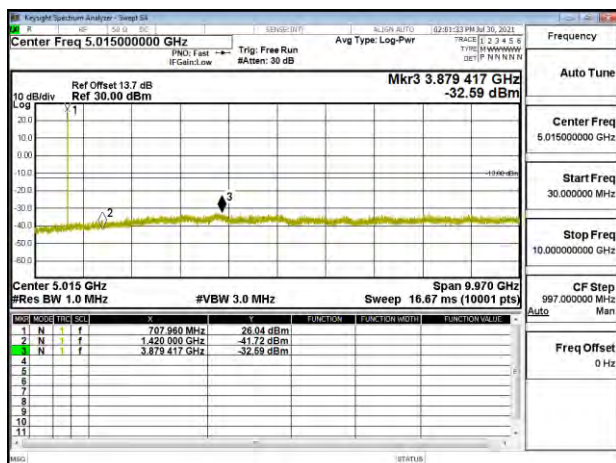
Band17_5MHz_QPSK_RB1_0_CH23790
