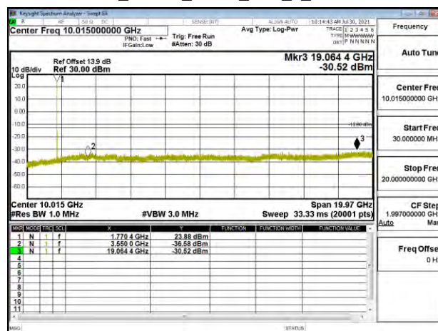
Band66_10MHz_QPSK_RB1_0_CH132622
