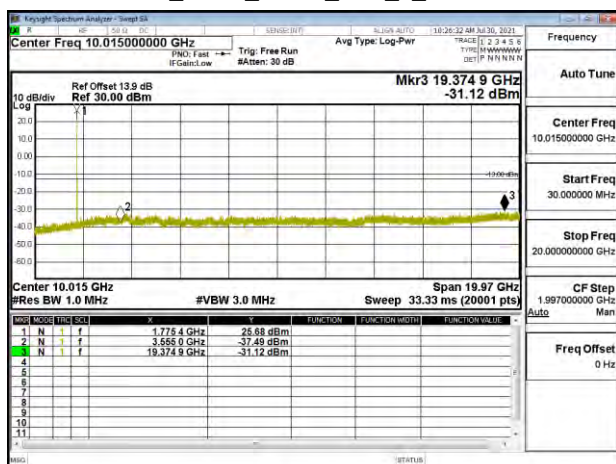
Band66_5MHz_QPSK_RB1_0_CH132647
