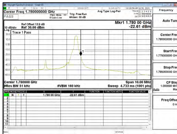
Band Edge_Band66_5MHz_QPSK_RB1_24_CH132647
