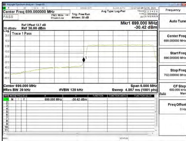
Band Edge_Band12_3MHz_QPSK_RB15_0_CH23025
