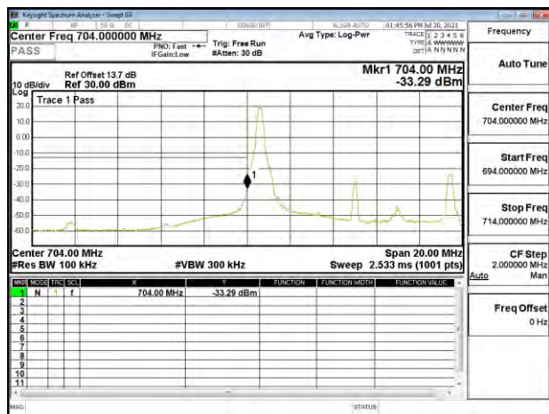
Band Edge_Band17_10MHz_QPSK_RB1_0_CH23780
