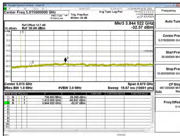
Band12_3MHz_QPSK_RB1_0_CH23095
