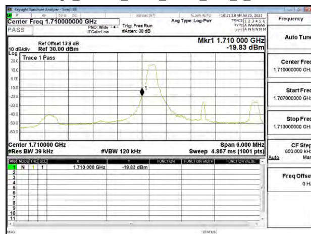
Band Edge_Band66_3MHz_QPSK_RB1_0_CH131987
