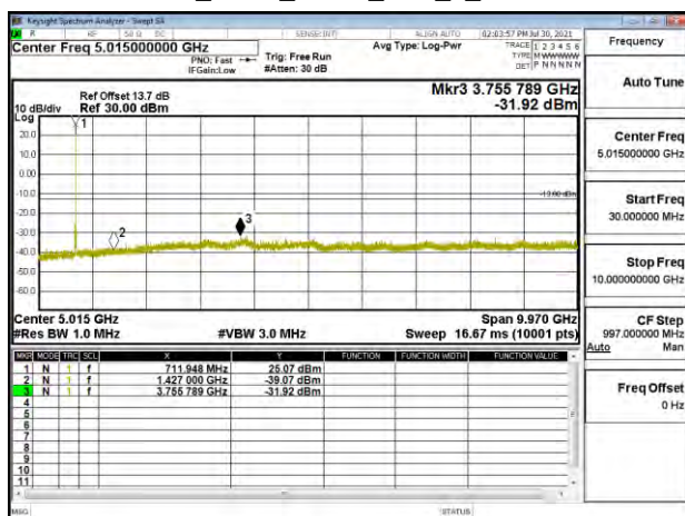
Band17_5MHz_QPSK_RB1_0_CH23825
