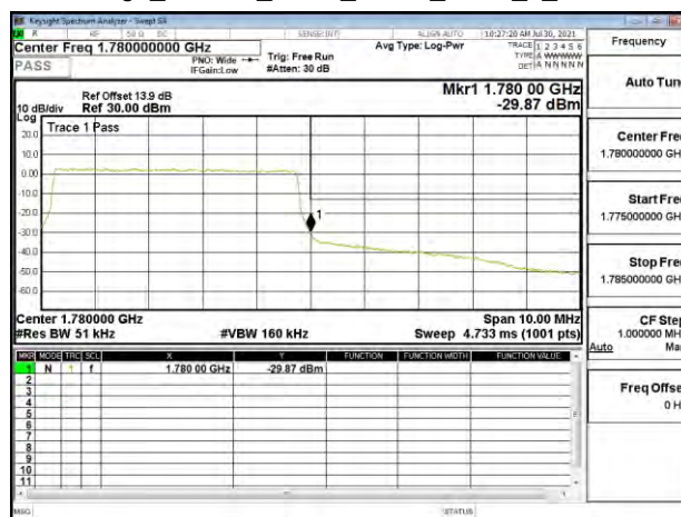
Band Edge_Band66_5MHz_QPSK_RB25_0_CH132647
