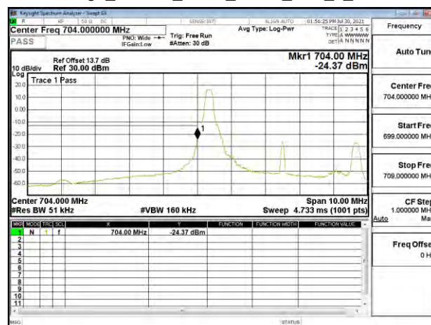
Band Edge_Band17_5MHz_QPSK_RB1_0_CH23755
