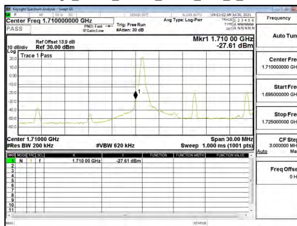
Band Edge_Band4_15MHz_QPSK_RB1_0_CH20025
