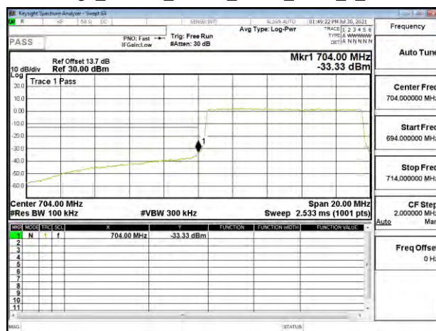
Band Edge_Band17_10MHz_QPSK_RB50_0_CH23780
