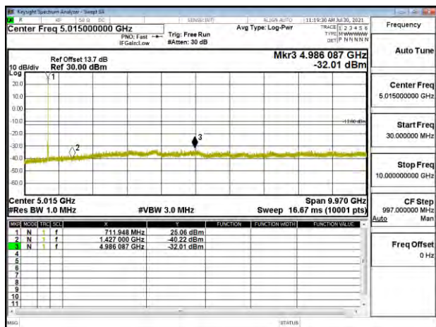
Band12_5MHz_QPSK_RB1_0_CH23155
