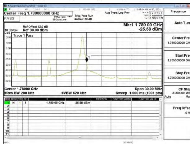
Band Edge_Band66_15MHz_QPSK_RB1_74_CH132597
