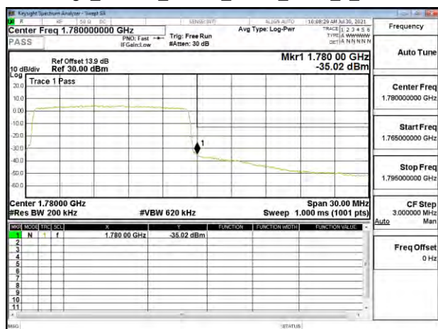
Band Edge_Band66_15MHz_QPSK_RB75_0_CH132597
