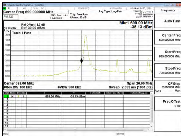
Band Edge_Band12_10MHz_QPSK_RB1_0_CH23060
