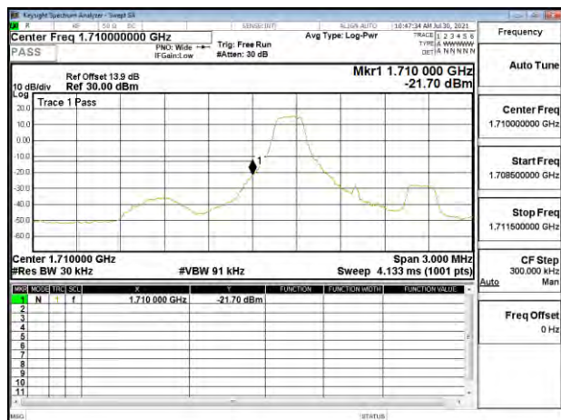
Band Edge_Band66_1.4MHz_QPSK_RB1_0_CH131979
