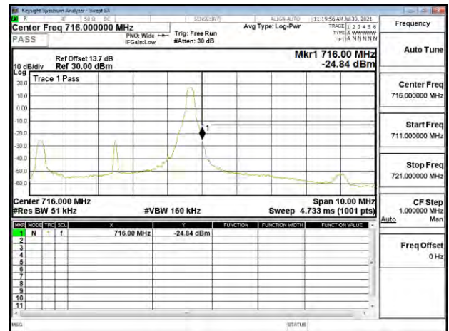
Band Edge_Band12_5MHz_QPSK_RB1_24_CH23155
