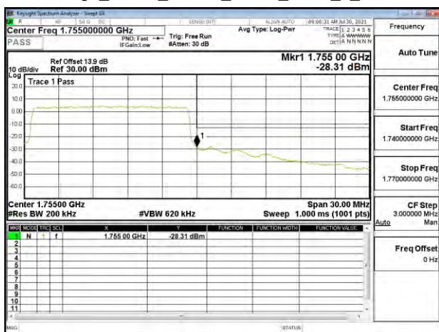
Band Edge_Band4_15MHz_QPSK_RB75_0_CH20325
