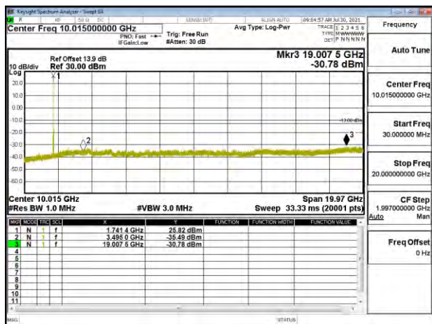
Band4_15MHz_QPSK_RB1_0_CH20325
