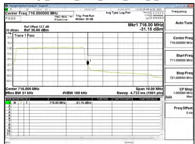
Band Edge_Band12_5MHz_QPSK_RB25_0_CH23155
