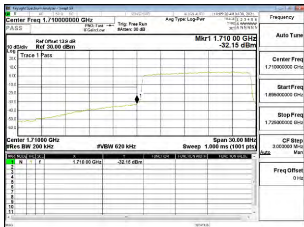
Band Edge_Band66_15MHz_QPSK_RB75_0_CH132047
