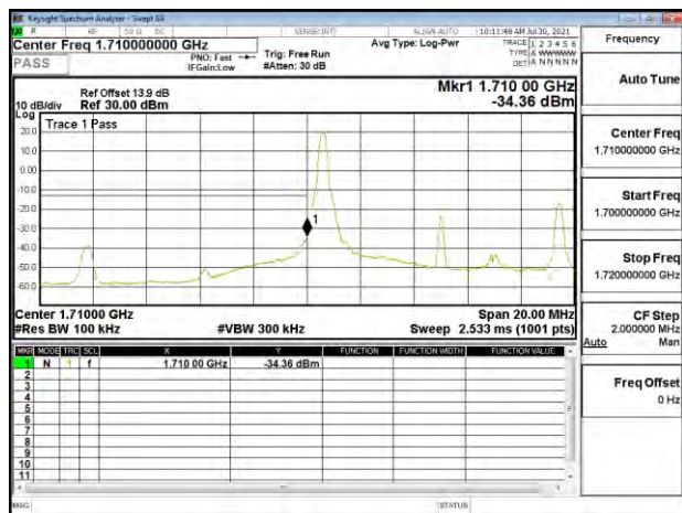
Band Edge_Band66_10MHz_QPSK_RB1_0_CH132022
