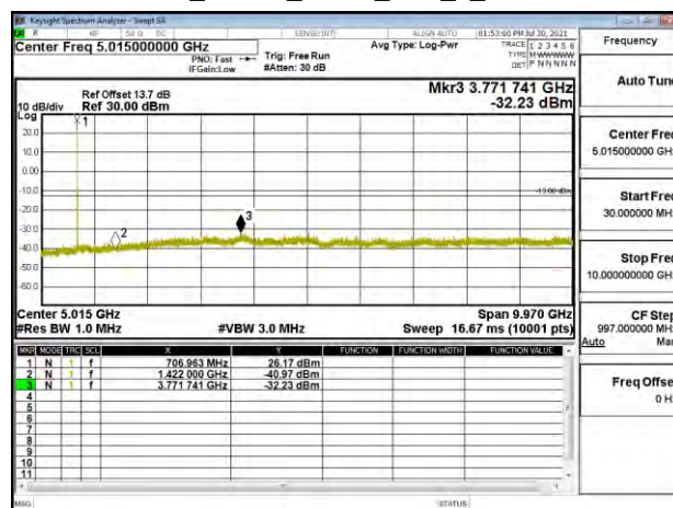
Band17_10MHz_QPSK_RB1_0_CH23800
