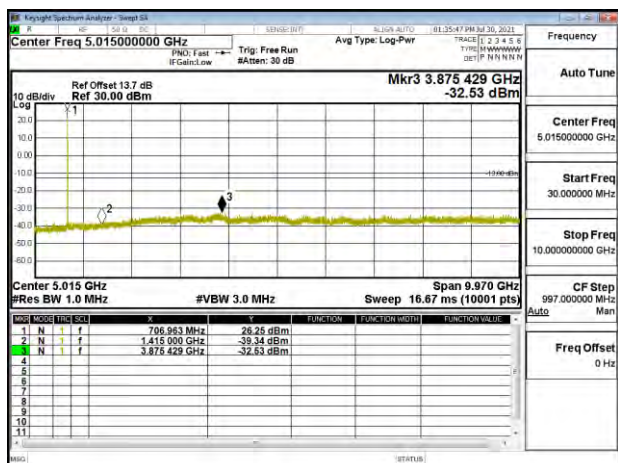
Band12_1.4MHz_QPSK_RB1_0_CH23095
