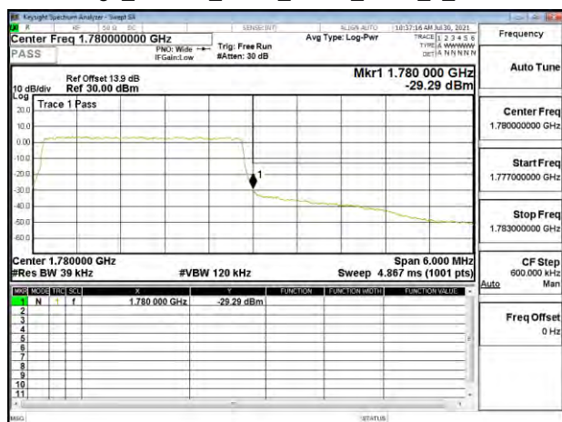
Band Edge_Band66_3MHz_QPSK_RB15_0_CH132657
