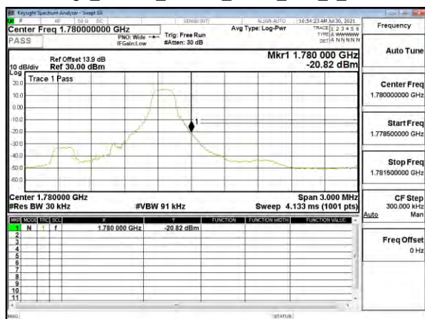
Band Edge_Band66_1.4MHz_QPSK_RB1_5_CH132665
