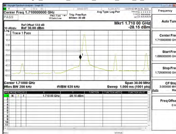
Band Edge_Band66_15MHz_QPSK_RB1_0_CH132047
