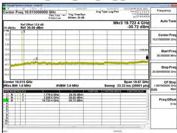
Band66_1.4MHz_QPSK_RB1_0_CH132665
