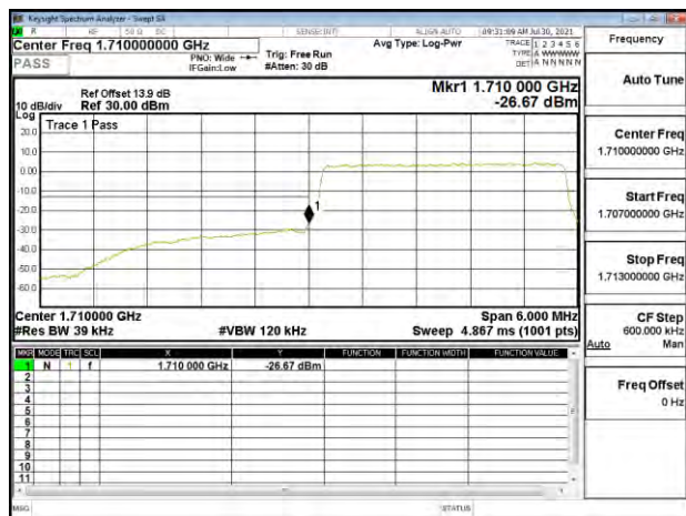
Band Edge_Band4_3MHz_QPSK_RB15_0_CH19965
