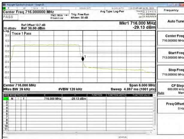
Band Edge_Band12_3MHz_QPSK_RB15_0_CH23165
