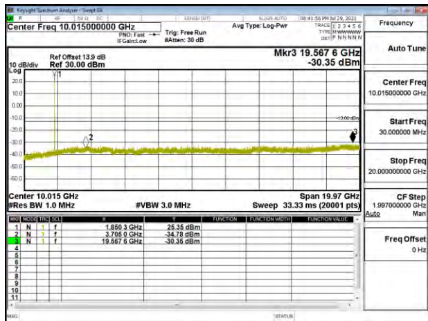
Band2_5MHz_QPSK_RB1_0_CH18900
