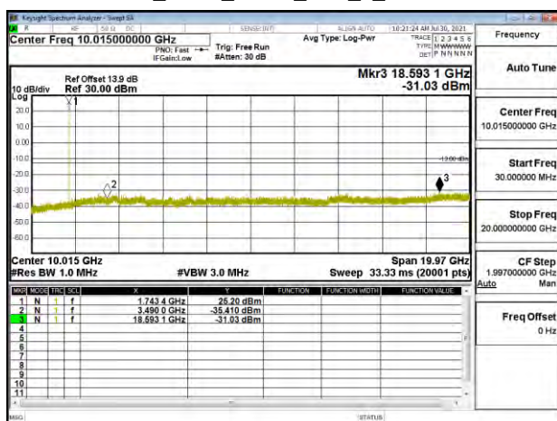
Band66_5MHz_QPSK_RB1_0_CH132322
