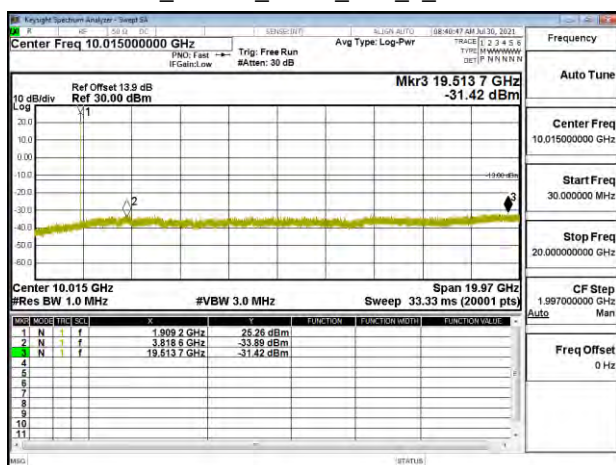
Band2_1.4MHz_QPSK_RB1_0_CH19193
