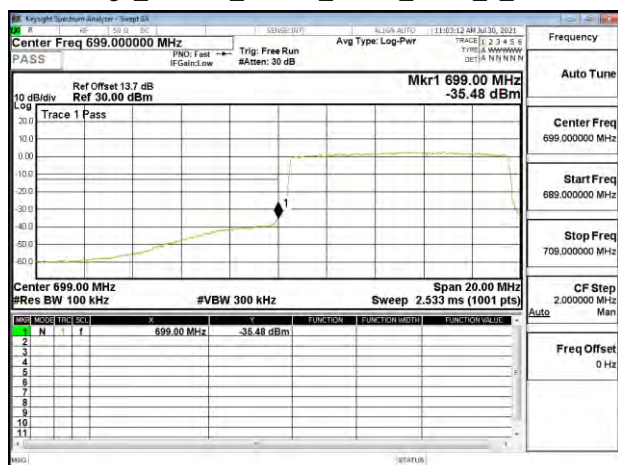
Band Edge_Band12_10MHz_QPSK_RB50_0_CH23060
