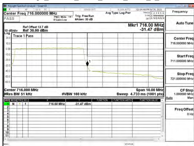
Band Edge_Band17_5MHz_QPSK_RB25_0_CH23825
