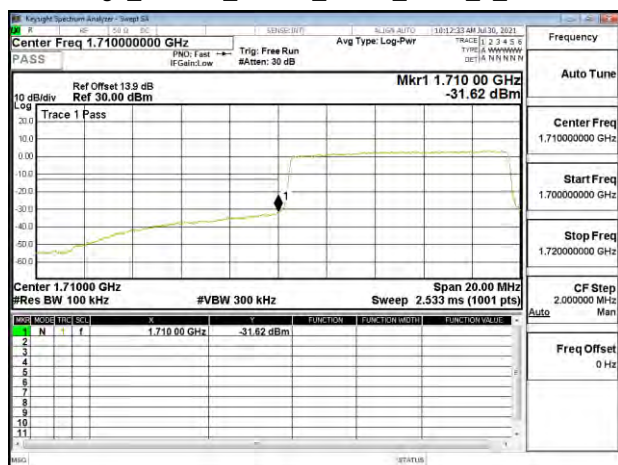
Band Edge_Band66_10MHz_QPSK_RB50_0_CH132022
