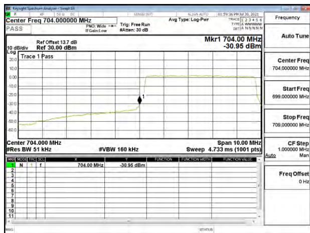
Band Edge_Band17_5MHz_QPSK_RB25_0_CH23755
