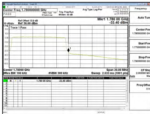
Band Edge_Band66_10MHz_QPSK_RB50_0_CH132622
