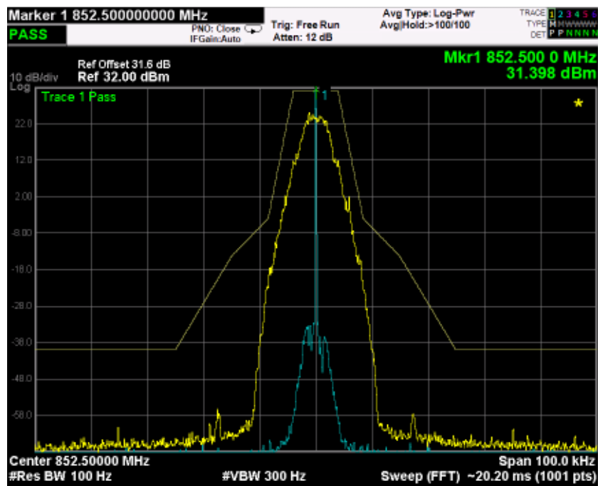
Mask H
