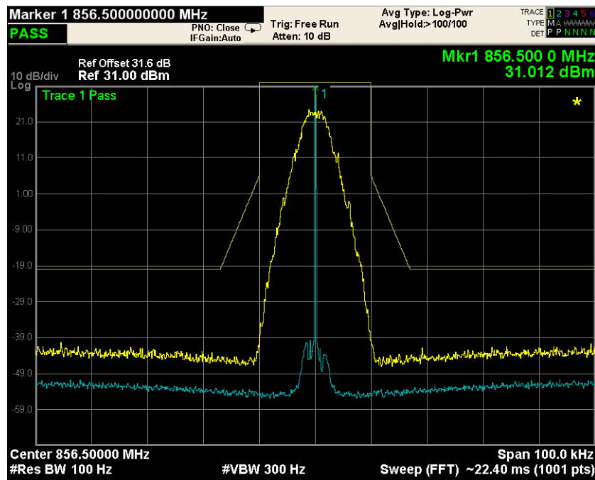
Mask G
