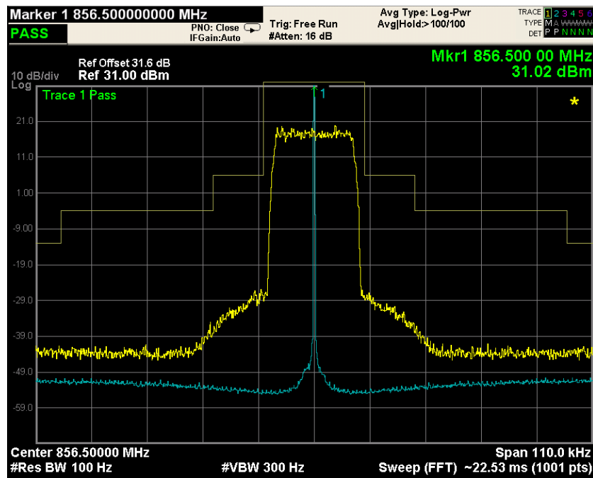
Mask B
