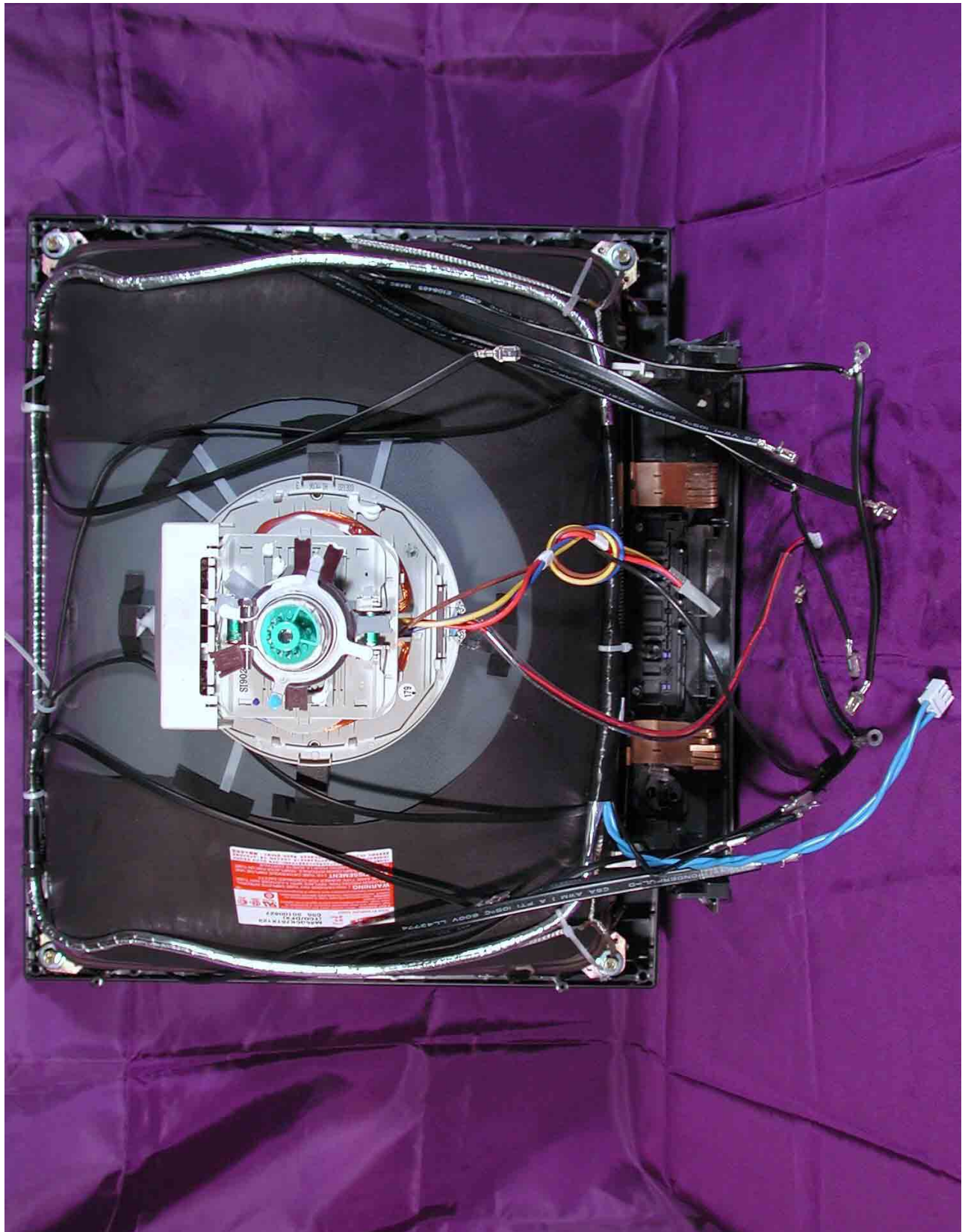
CRT Assembly
