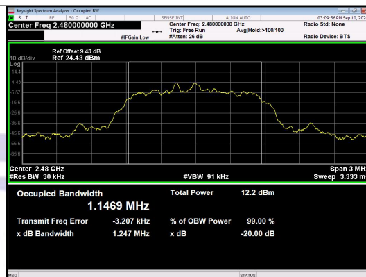
n/4DQPSK_2-DH1_Channel 78
