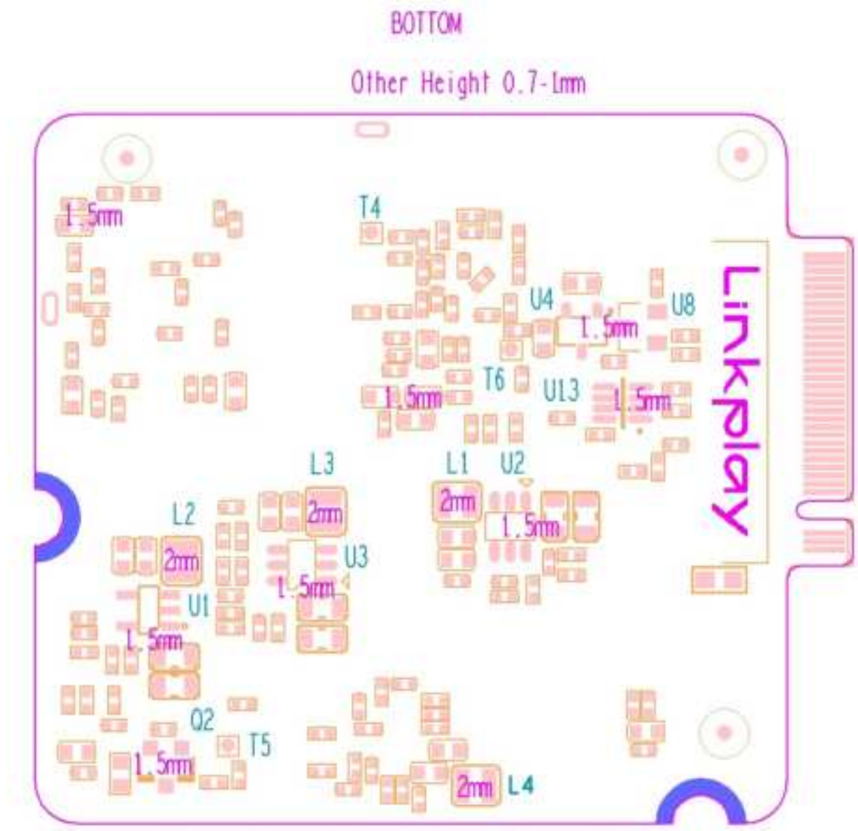
Figure 2-2 A98M Physical Dimension
