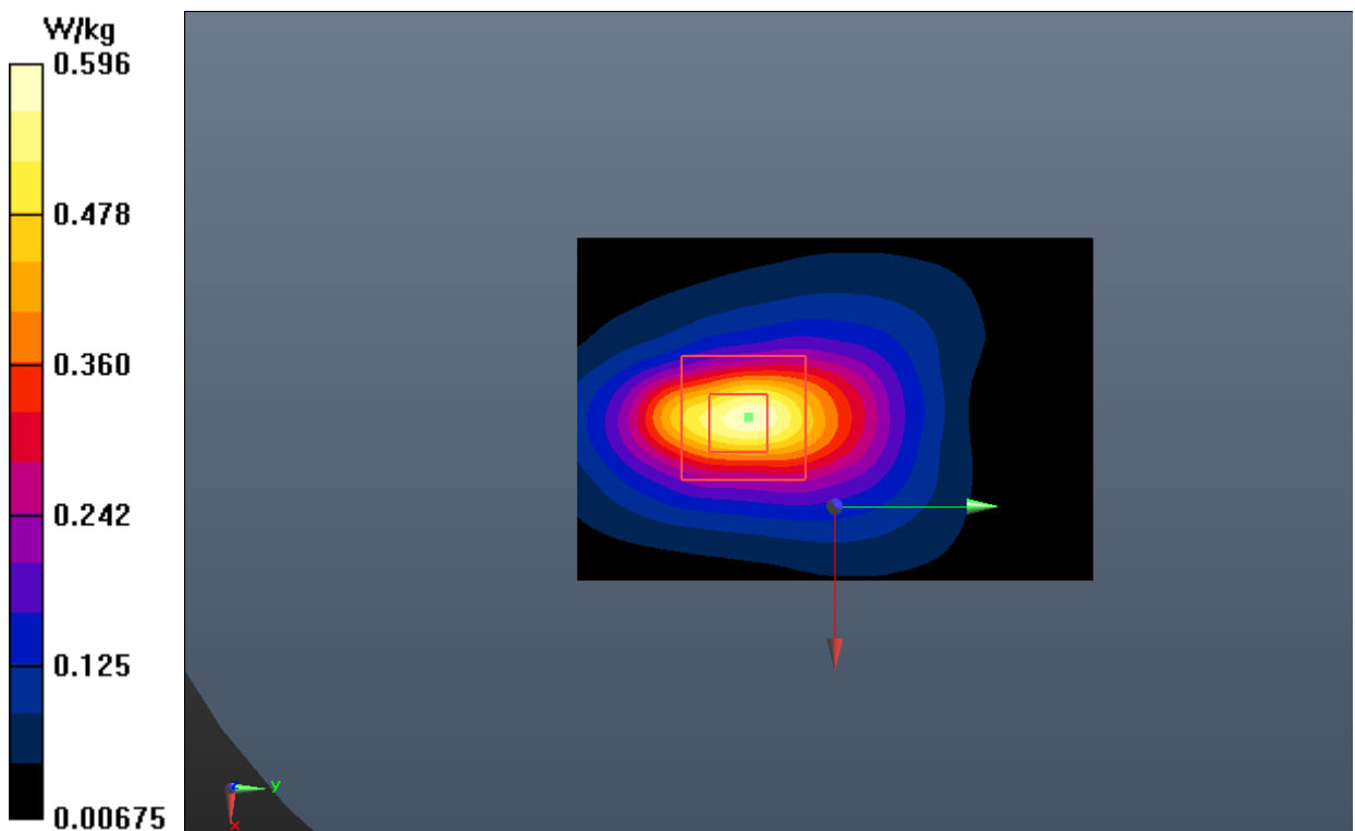
Fig.4 GSM 1900 Body
