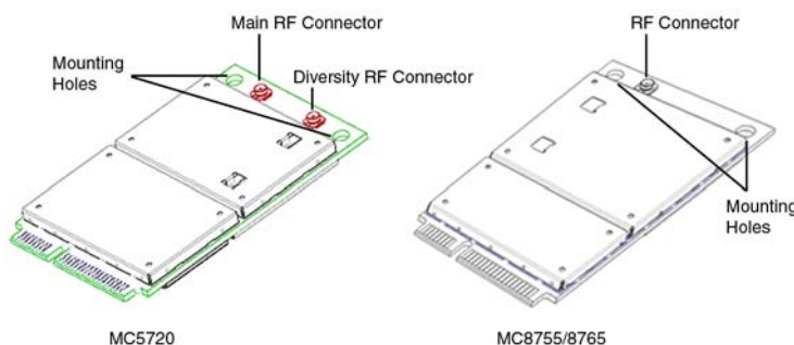
Figure 3-1: Antenna connection points and mounting holes
