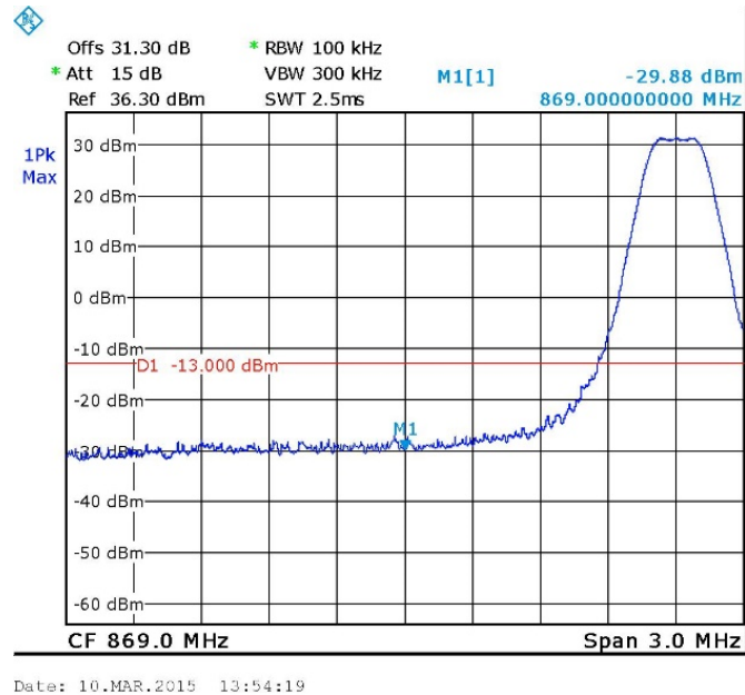
Figure 51. — GSM - 870.20 MHz
