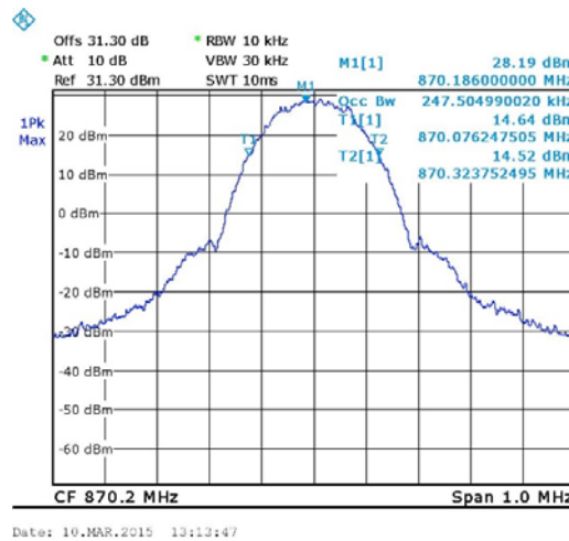
Figure 26. — GSM - Output 870.20MHz
