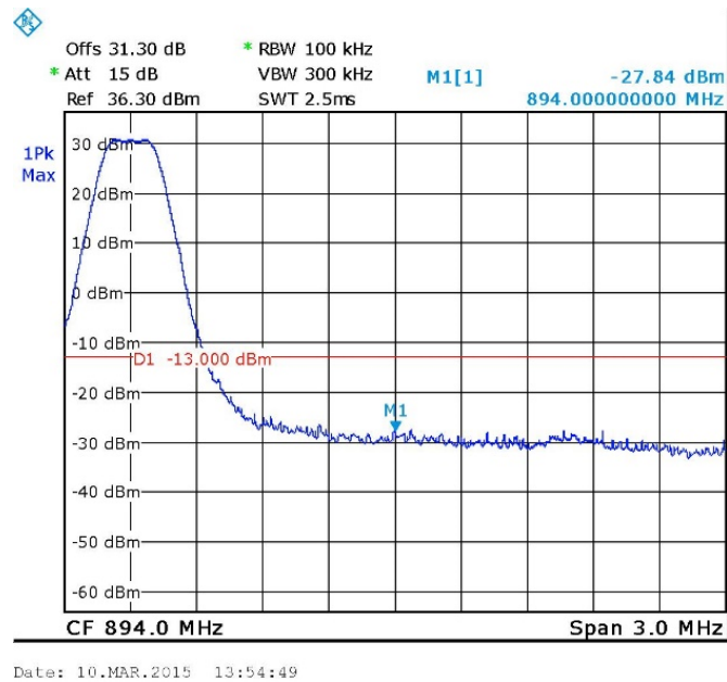
Figure 52. — GSM - 892.80 MHz
