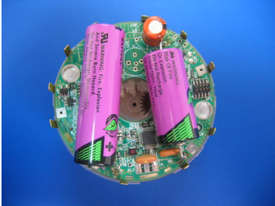
Photograph No.2 ETMW water reader PCB component side with batteries
