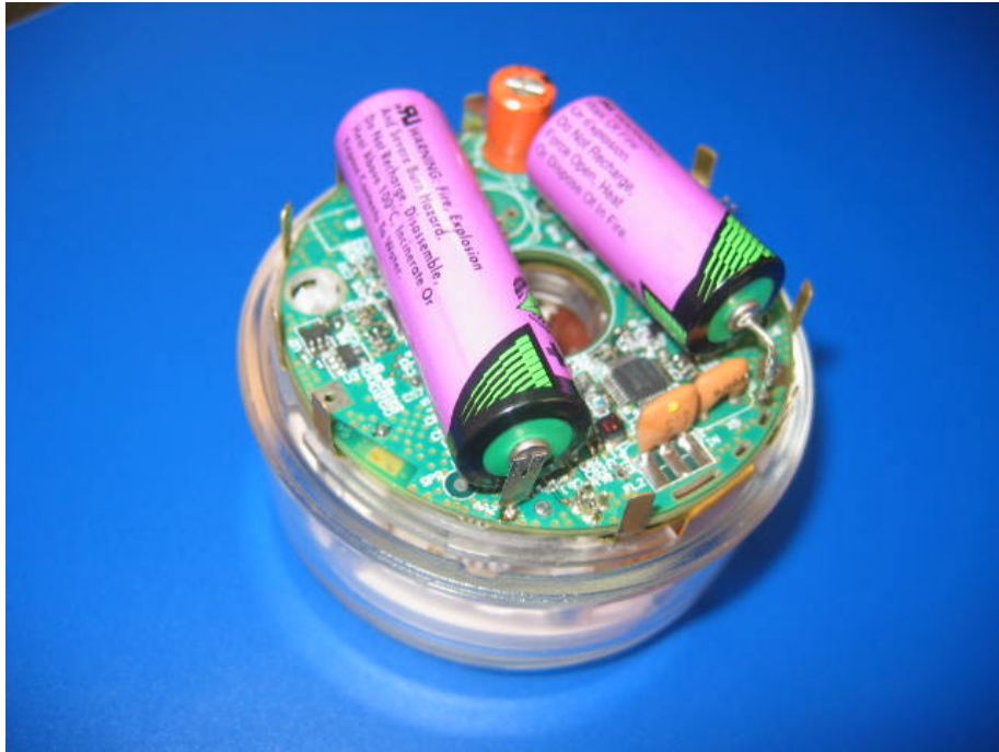
Photograph No.1 ETMW water reader Internal view
